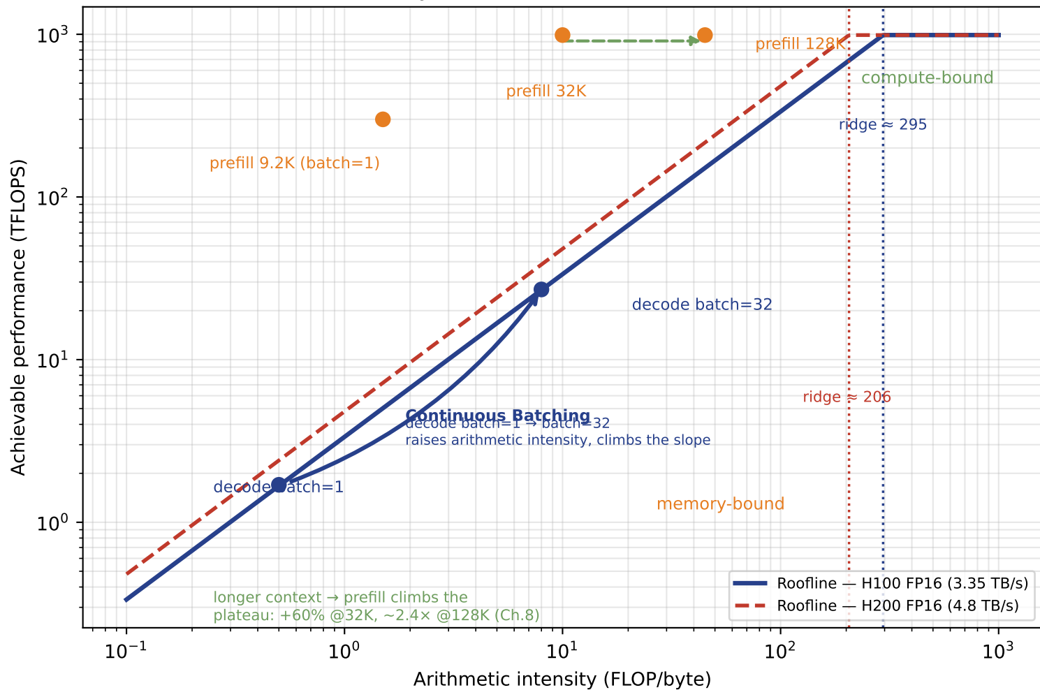
Arithmetic-intensity roofline — 70B FP16 on 8×H100 / 8×H200
