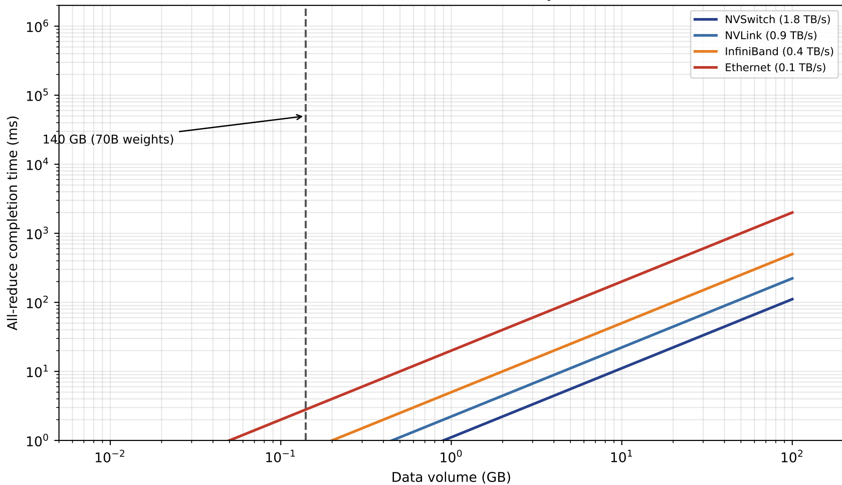
Ch09 — all-reduce time vs data volume, by interconnect tier
