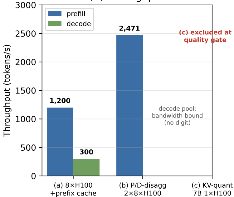
(2) Throughput
