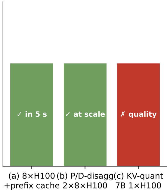
(3) Constraint verdict
