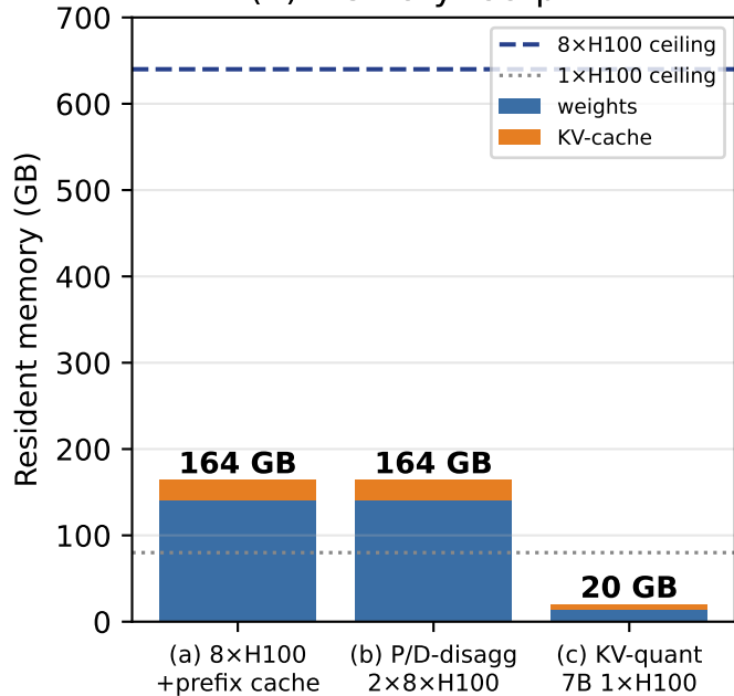
(1) Memory footprint
