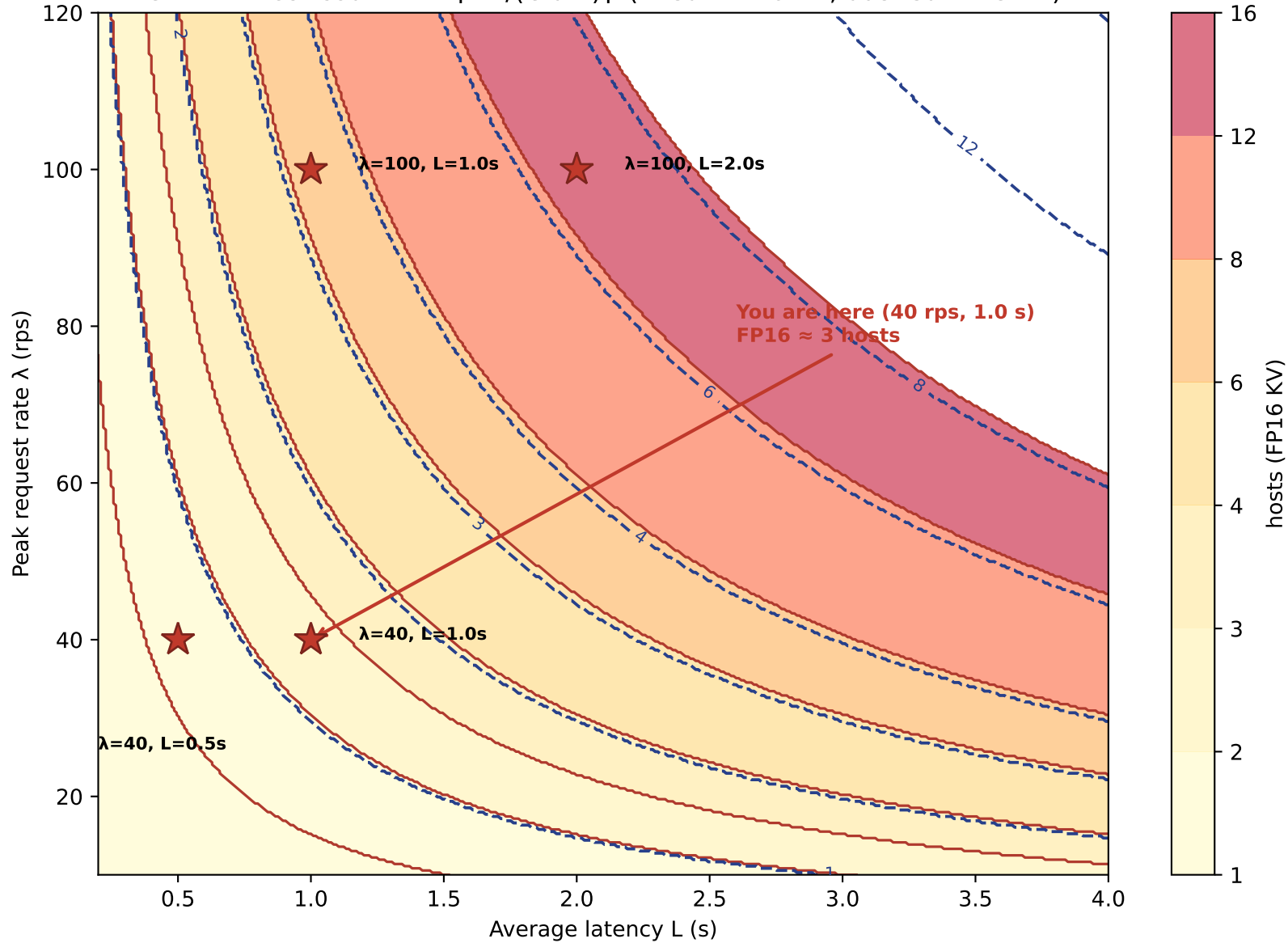
Ch17 — host count H = \lceil \lambda \cdot L / (C \cdot \text{util}) \rceil (filled=FP16 KV, dashed=FP8 KV)
