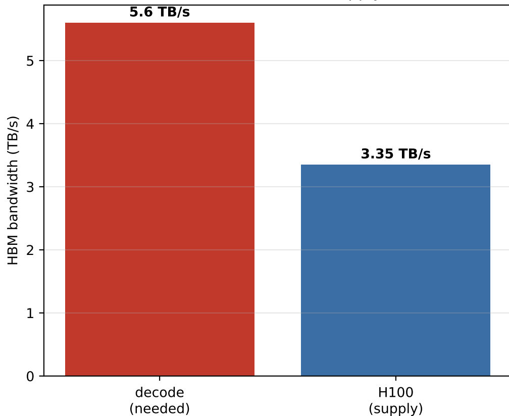
Decode: HBM-bandwidth-bound (5.6 needed > 3.35 supply)
