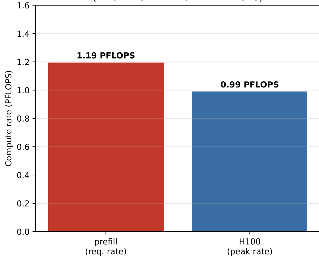
Prefill: compute-bound \rightarrow required rate (1.29 PFLOP \div \sim 1 s \approx 1.2 PFLOPS)
