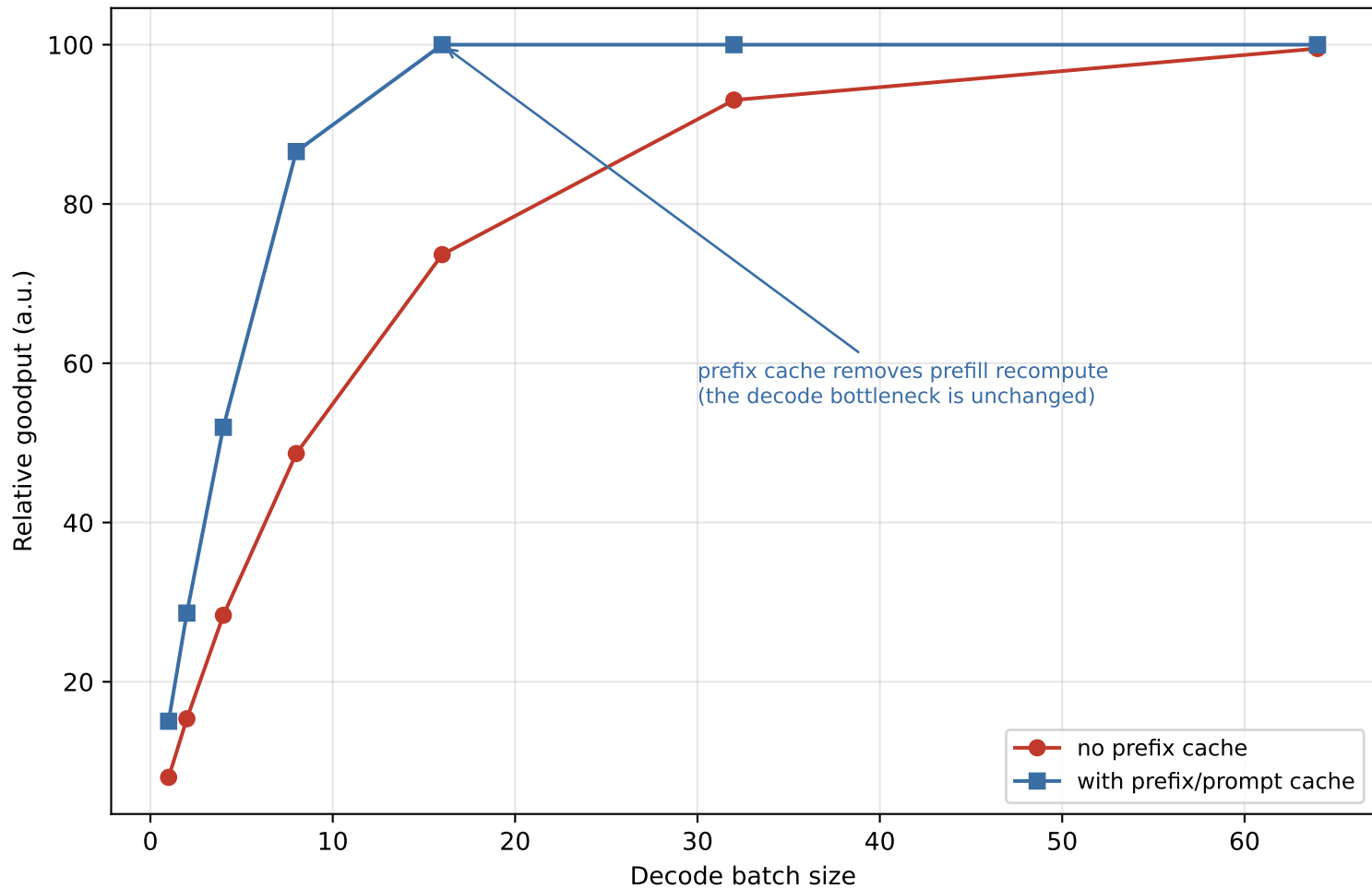
Ch15 — batching raises decode goodput; prefix cache raises the ceiling
