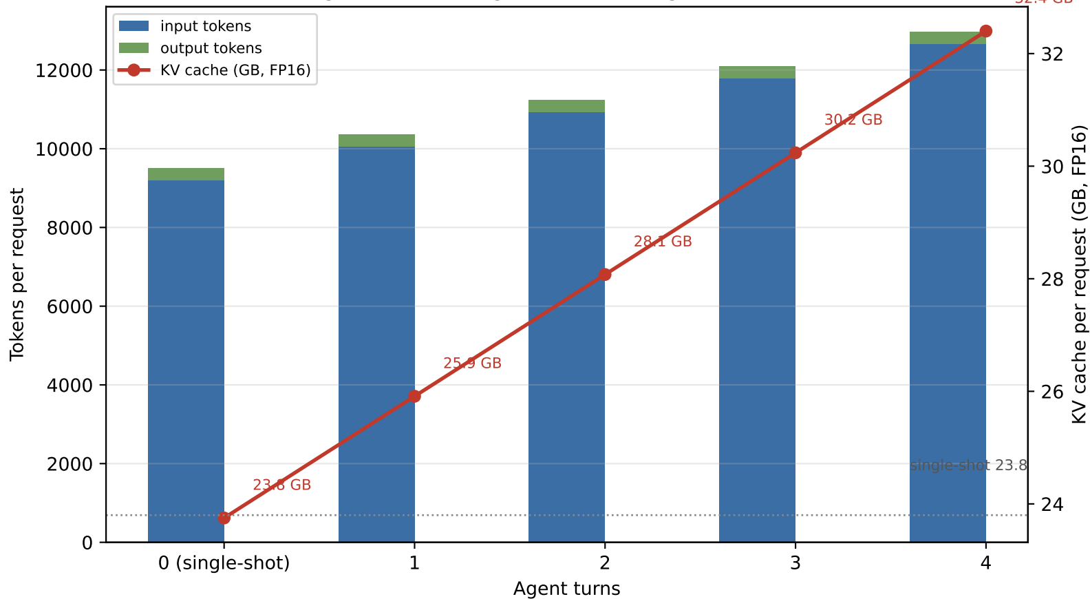
Ch19 — token growth and KV growth across agent turns (23.8 → 32.4 GB)
