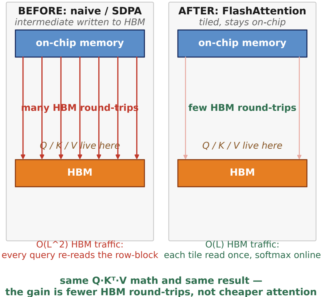
FIGURE 15.1: FlashAttention: the same math, far less HBM traffic. Before (naive / SDPA), the intermediate attention matrix is materialized to HBM and re-read, so every query block re-streams the full K/V row-block — many HBM round-trips. After (FlashAttention), the computation is tiled and fused so the K/V tiles stream through on-chip memory once and the result is accumulated in place — few HBM round-trips. The attention result is identical; the gain is fewer HBM round-trips, not a change to the attention mathematics. [ILLUSTRATIVE conceptual]
