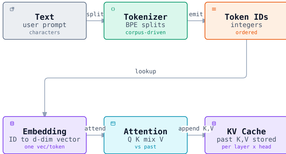
FIGURE 1.2: How a token travels: text \rightarrow tokenizer \rightarrow IDs \rightarrow embedding \rightarrow attention \rightarrow KV cache [ILLUSTRATIVE conceptual]
