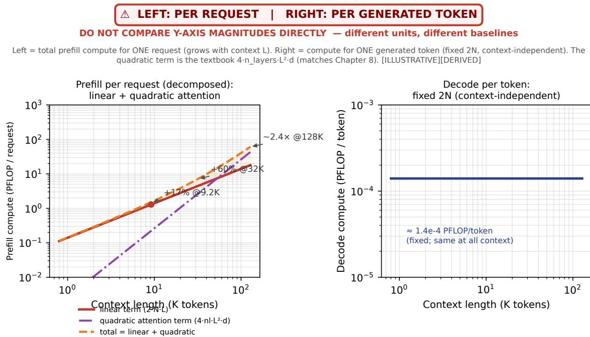
FIGURE 22.1: Full-attention prefill increasingly reflects quadratic attention cost; decode is incurred token-by-token. Two aligned panels (different units, not directly comparable): LEFT = prefill PER REQUEST (linear 2NL vs linear+quadratic 4 \cdot n_{\text{layers}} \cdot L^2 \cdot d ; +17% @ 9.2K, +60% @ 32K, \sim 2.4 \times @ 128K); RIGHT = decode PER TOKEN (fixed 2N \approx 1.4e-4 PFLOP/token, flat across context). The quadratic term is the textbook 4 \cdot n_{\text{layers}} \cdot L^2 \cdot d and matches Chapter 8 [ILLUSTRATIVE][DERIVED]
