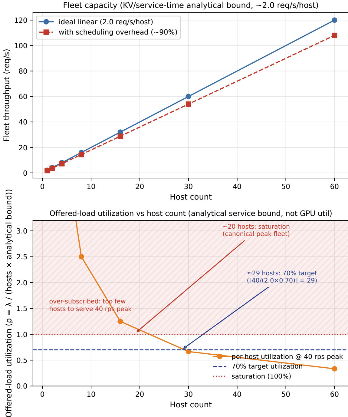
FIGURE 20.1: Fleet capacity (KV/service-time analytical bound, ~2.0 req/s/host) and per-host utilization, vs. host count at the canonical peak load (40 rps). Top panel: capacity against host count from the KV/service-time analytical bound (~2.0 req/s/host), with a ~90% scheduling-overhead line. Bottom panel: per-host utilization at the canonical 40 rps peak. This is the honest quantity for the tail: p99 is driven by per-host utilization, not by host count alone . Adding hosts lowers per-host utilization (more headroom) hence lowers the expected tail; the 70%-utilization and 100%-saturation reference lines show the provisioning target. The tail also depends on the arrival process, scheduling policy, batching, and the service-time distribution, which a provisioning model alone does not capture. The ~2.0 req/s line is the KV/service-time analytical bound, not a benchmarked serving throughput. [ILLUSTRATIVE][DERIVED]
