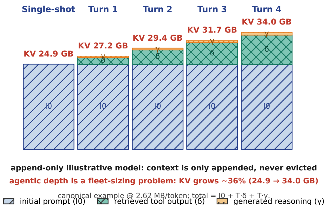
FIGURE 19.3: The agentic context block grows every turn: initial prompt (9.2K tok) plus tool output (δ) + reasoning (γ) appended each turn, FP16 KV footprint rising 24.9 → 34.0 GB (max-KV, end-of-request). This schematic shows the mechanism — the initial prompt base plus cumulative tool-output and reasoning blocks. (Companion Fig 19.2 quantifies the total.) [ILLUSTRATIVE][DERIVED: Ch19 arithmetic]
