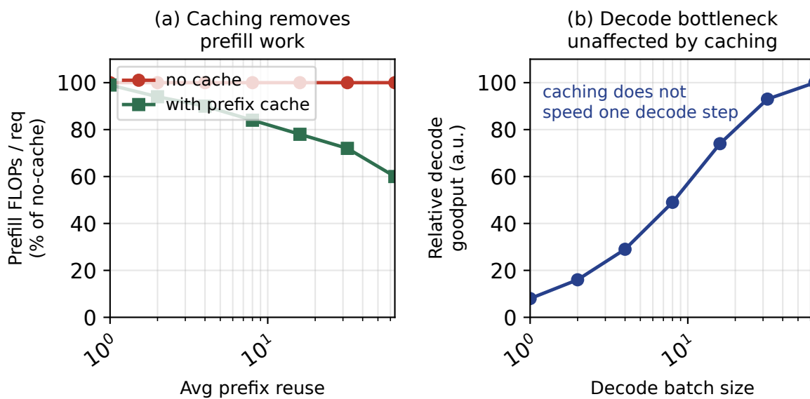
FIGURE 15.2: Prefix caching and batching affect different serving phases: caching reduces prefill work; batching raises decode goodput
