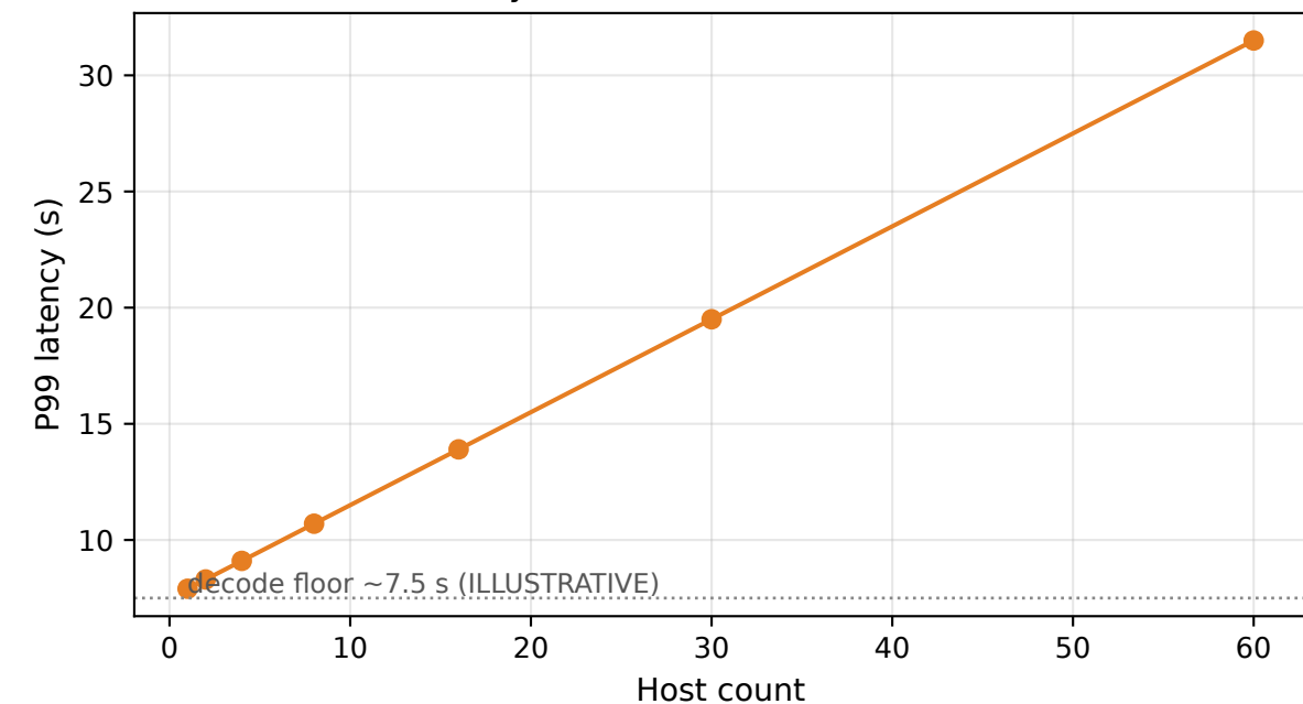
P99 latency vs host count (decode-dominated)
