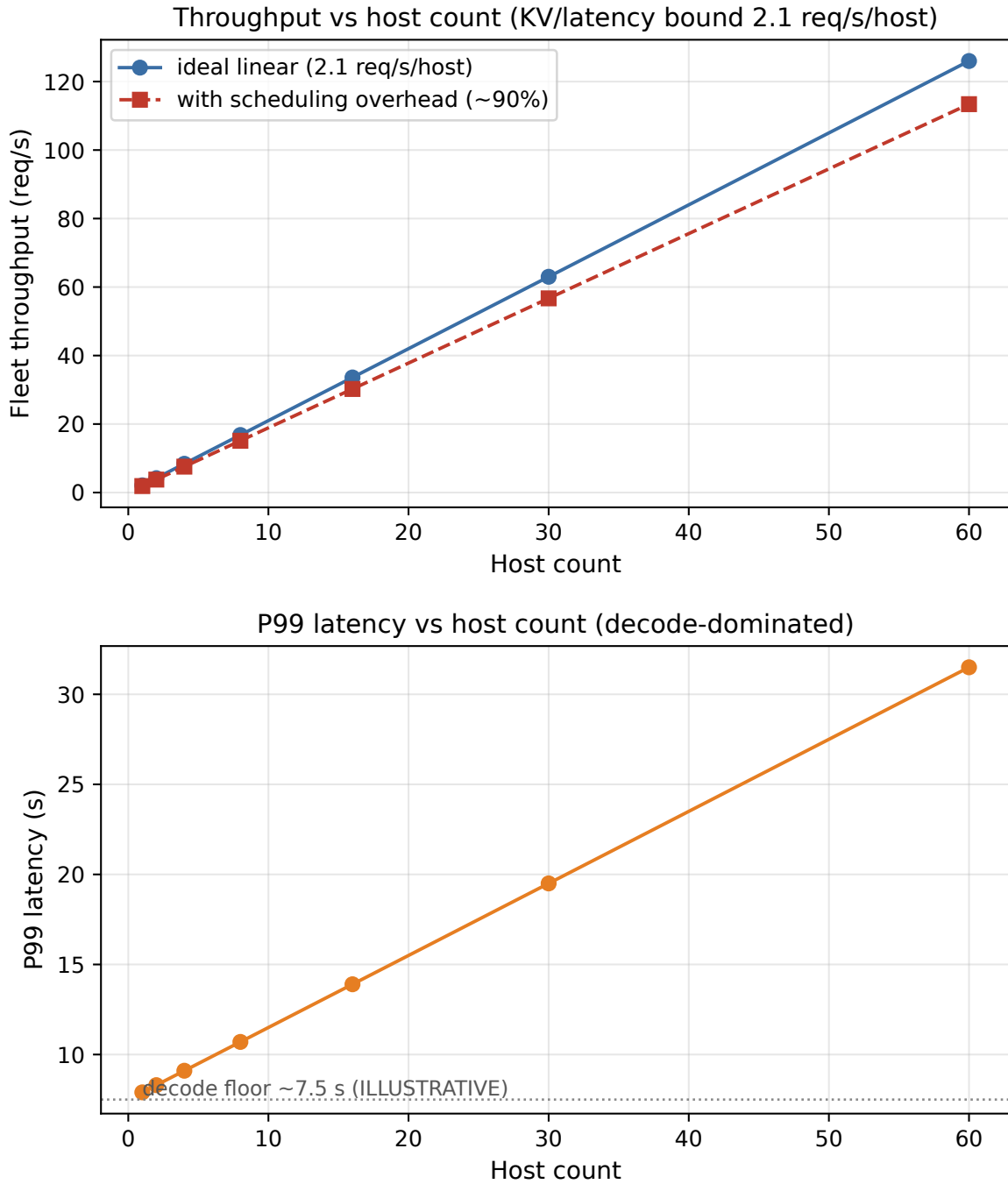
FIGURE 20.1: Fleet QPS and latency vs. host count, batch size, and scheduling overhead. The throughput panel is model-derived (KV/latency bound \sim 2.1 req/s/host, shown with a \sim 90\% scheduling-overhead line); the p99 panel is explicitly illustrative, using a decode floor \sim 7.5 s plus a heuristic queueing term — host count alone does not determine p99 without arrival, scheduling, batching, and queueing assumptions [ILLUSTRATIVE][DERIVED]
