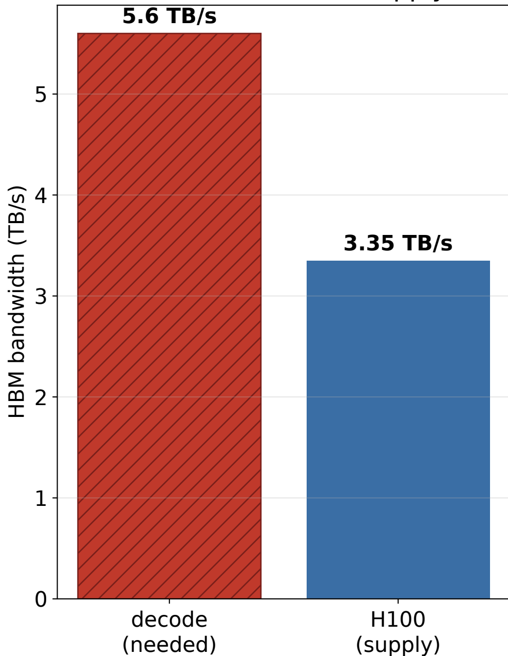
Decode: HBM-bandwidth-bound (5.6 needed > 3.35 supply)
