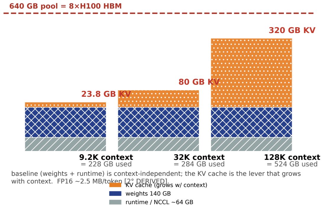
FIGURE 7.5: Memory Tetris: how the 8xH100 host's 640 GB pool fills at three contexts (9.2K / 32K / 128K). Runtime \sim 64 GB + weights 140 GB + KV cache 23.8 / 80 / 320 GB [2° DERIVED]
