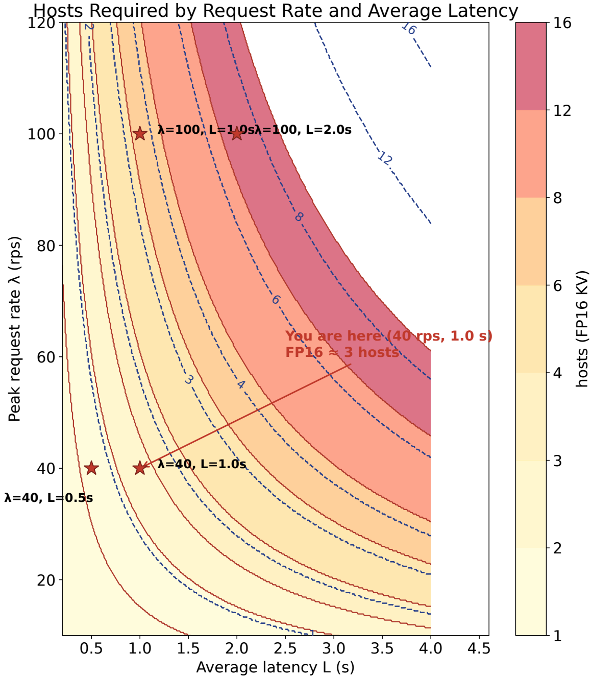
FIGURE 17.2: Hosts required by request rate and average latency, with the FP16-KV family ( C \approx 18 , filled) and the FP8-KV family ( C \approx 33 , dashed). Each contour is a fixed integer host count, H = \text{ceil}(\lambda_{\text{peak}} * L / (C * \text{util})) [DERIVED: Ch17 §3 + Ch7 KV constants]
