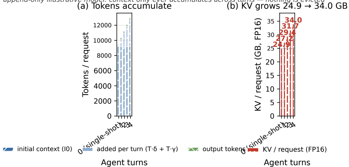
FIGURE 19.2: Input/output tokens and KV cache per request across agent turns ( I_0 + T \cdot \delta + T \cdot \gamma ; 9,200 + 800 + 65 per turn), FP16 KV rising from 24.9 GB single-shot to 34.0 GB at 4 turns. This chart quantifies the growth — the total token and KV numbers as turns accumulate. (Companion Fig 19.3 shows the mechanism of why it grows.) [DERIVED: Ch19 §3 arithmetic]
