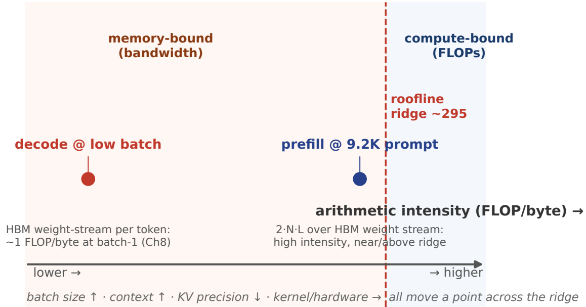
FIGURE 2.2: Prefill and decode sit on an arithmetic-intensity continuum, split by the roofline ridge. Low-batch decode (streaming weights per token) lands at ~1 FLOP/byte — the memory-bound side; long-prompt prefill lands at high intensity — the compute-bound side. These are operating points, not fixed identities: batch, context, precision, kernel and hardware all move a point across the ridge. [ILLUSTRATIVE conceptual, roofline developed in Ch 8]
