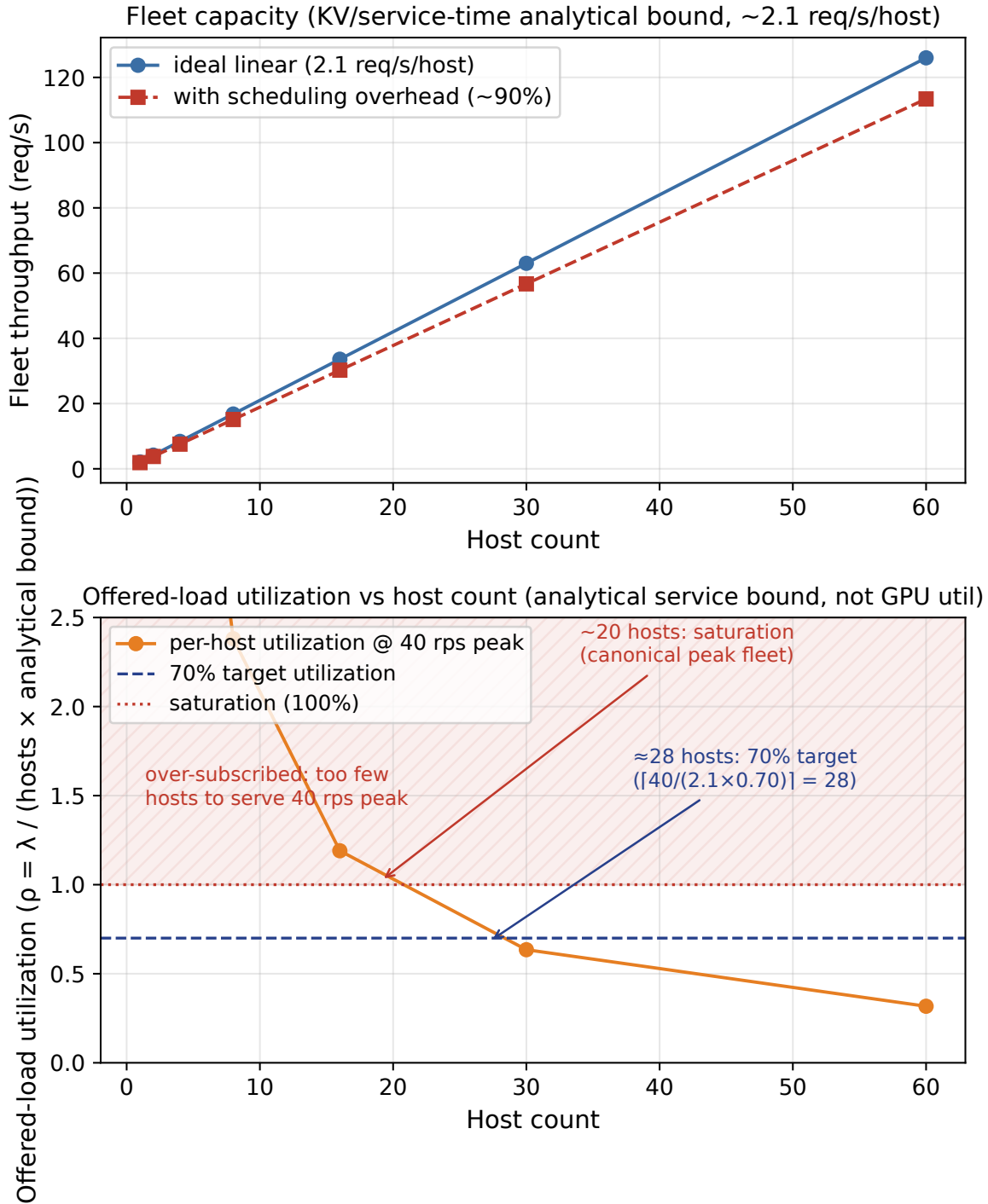
FIGURE 20.1: Fleet capacity (KV/service-time analytical bound, ~2.1 req/s/host) and per-host utilization, vs. host count at the canonical peak load (40 rps). Top panel: capacity against host count from the KV/service-time analytical bound (~2.1 req/s/host), with a ~90% scheduling-overhead line. Bottom panel: per-host utilization at the canonical 40 rps peak. This is the honest quantity for the tail: p99 is driven by per-host utilization, not by host count alone . Adding hosts lowers per-host utilization (more headroom) hence lowers the expected tail; the 70%-utilization and 100%-saturation reference lines show the provisioning target. The tail also depends on the arrival process, scheduling policy, batching, and the service-time distribution, which a provisioning model alone does not capture. The ~2.1 req/s line is the KV/service-time analytical bound, not a benchmarked serving throughput. [ILLUSTRATIVE][DERIVED]
