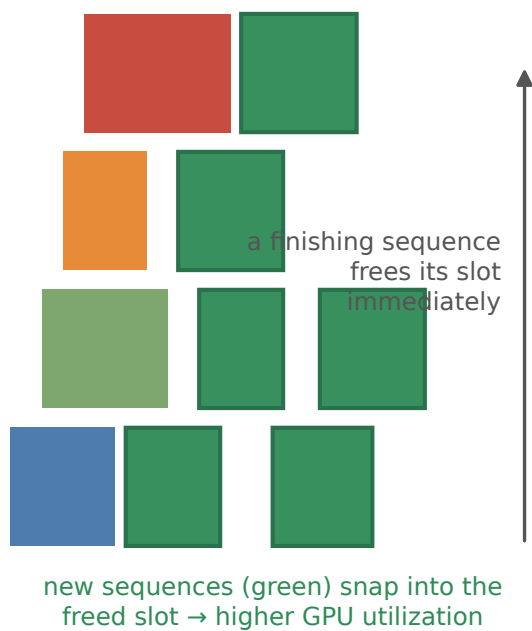
FIGURE 11.1: Discrete vs continuous batching (Orca-style slot diagram). Discrete batching runs each batch to completion, leaving GPU slots idle as sequences finish early; continuous batching admits and evicts requests at every decode step, backfilling freed slots (illustrative, after Orca, OSDI 2022)
