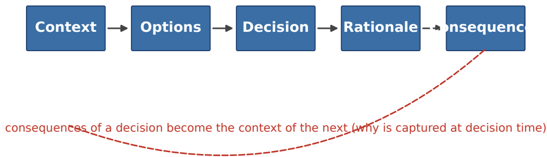
FIGURE 25.1: The Anatomy of an Architecture Decision Record
