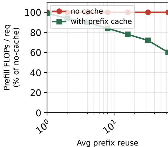
(a) Caching removes prefill work
