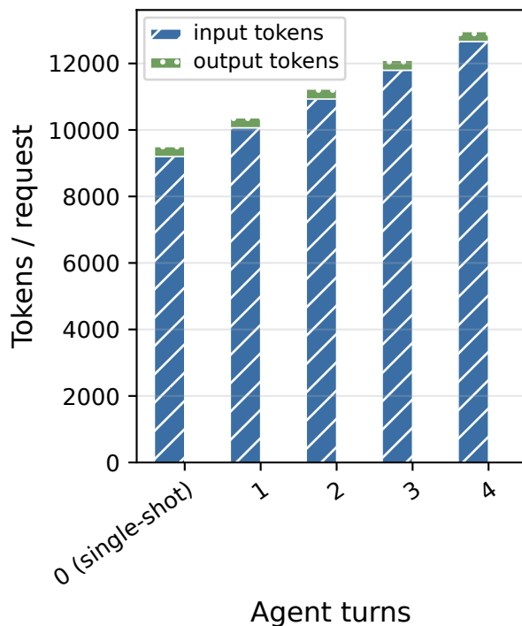
(a) Tokens accumulate
