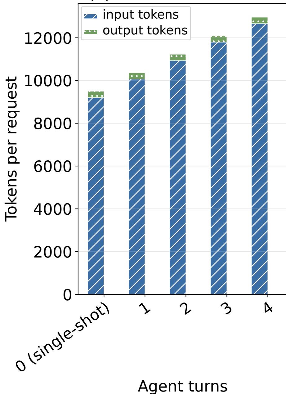
(a) Tokens accumulate
