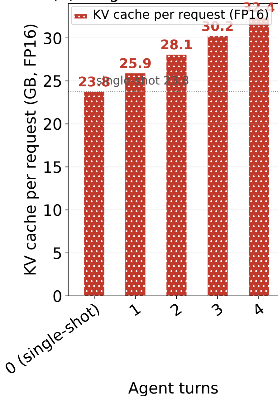
(b) KV grows 23.8 → 32.4 GB
