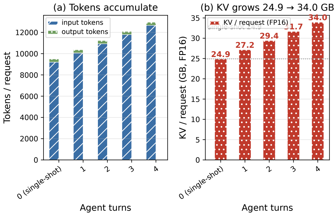
FIGURE 19.2: Input/output tokens and KV cache per request across agent turns ( I_0 + T \cdot \delta + T \cdot \gamma ; 9,200 + 800 + 65 per turn), FP16 KV rising from 24.9 GB single-shot to 34.0 GB at 4 turns. This chart quantifies the growth — the total token and KV numbers as turns accumulate. (Companion Fig 19.3 shows the mechanism of why it grows.) [DERIVED: Ch19 §3 arithmetic]
