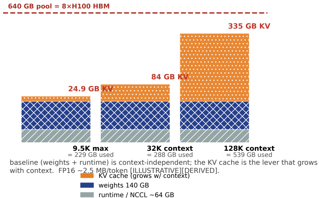
FIGURE 7.5: Memory Tetris: how the 8×H100 host’s 640 GB aggregate pool fills at three contexts (9.5K max / 32K / 128K). Runtime ~64 GB + weights 140 GB + KV cache 24.9 / 84 / 335 GB. Aggregate-feasibility caveat: this is an aggregate residency test on the 640 GB total, not a proof that each allocation maps cleanly onto per-rank HBM. Sharding, KV partitioning, fragmentation, and inter-connect topology must be validated per rank; “total bytes < total HBM” is a first-order screen, not a fit guarantee. [ILLUSTRATIVE][DERIVED]
