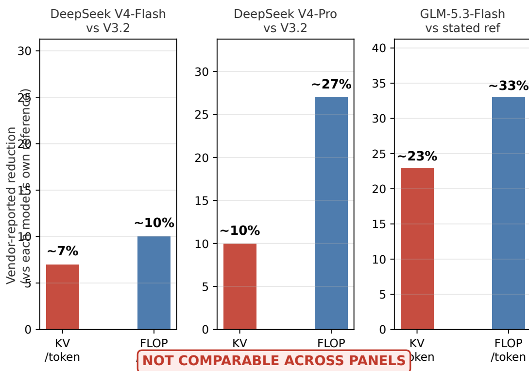
FIGURE A.2: Vendor-reported KV/FLOP reduction relative to each model's stated predecessor/reference, not a cross-model baseline [DERIVED from 1P claims: arXiv 2606.19348; HF zai-org]
