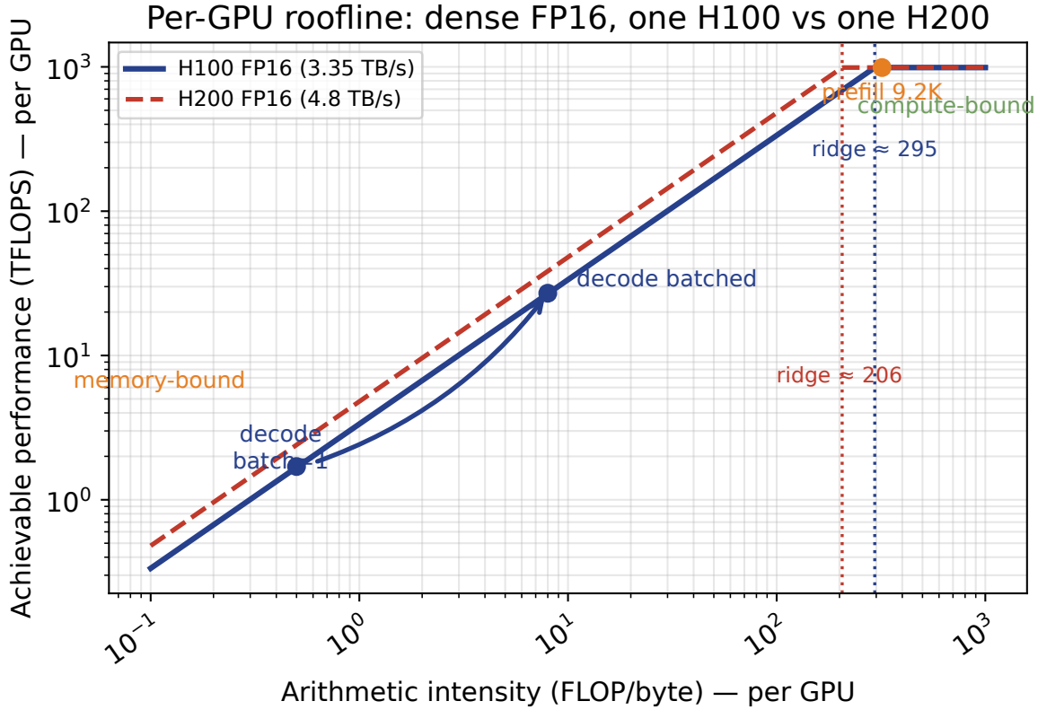
FIGURE 8.1: Per-GPU roofline for dense FP16, one H100 vs one H200 (a per-GPU chart, not a host-level one). Compute ceiling and HBM bandwidth are single-GPU quantities here (989 TFLOPS, 3.35 / 4.8 TB/s), so the ridge point and the memory-bound slope are per-GPU. Prefill (9.2K input) sits to the right of the ridge, on the compute-bound plateau; decode (batch=1) sits to the left, on the memory-bound slope, and continuous batching climbs the slope as batch grows. The ridge classification (compute-vs memory-bound) is unchanged by ideal N-way replication because both peak FLOP/s and HBM bandwidth scale with GPU count; host-level attainable performance additionally depends on sharding and communication. [DERIVED from 1P: vendor datasheet]
