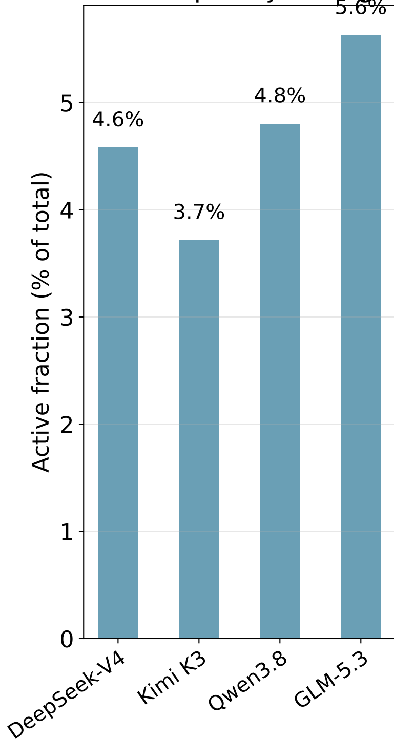
Frontier MoE total vs active parameters — single digits
