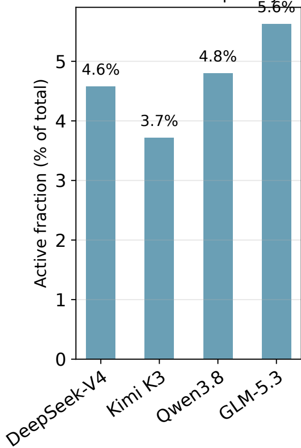
Extreme MoE sparsity
