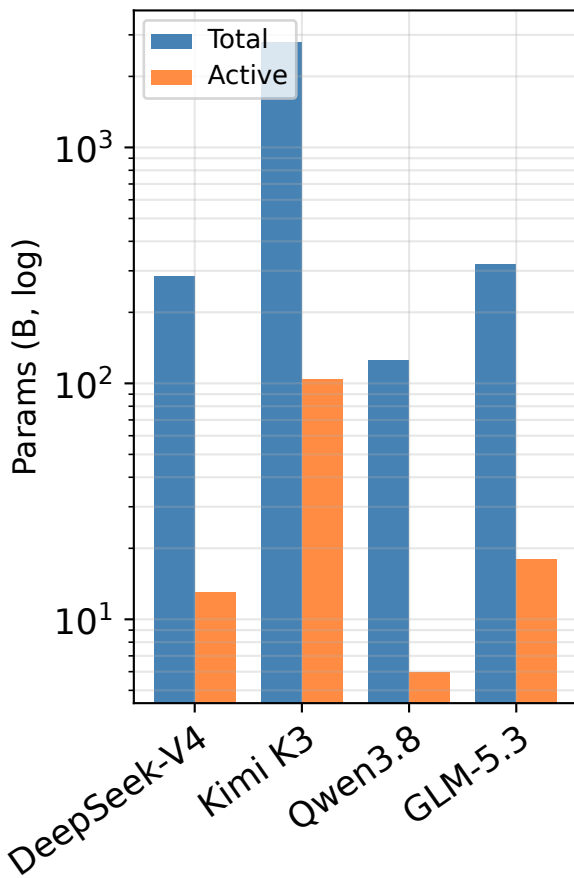
Total vs active
