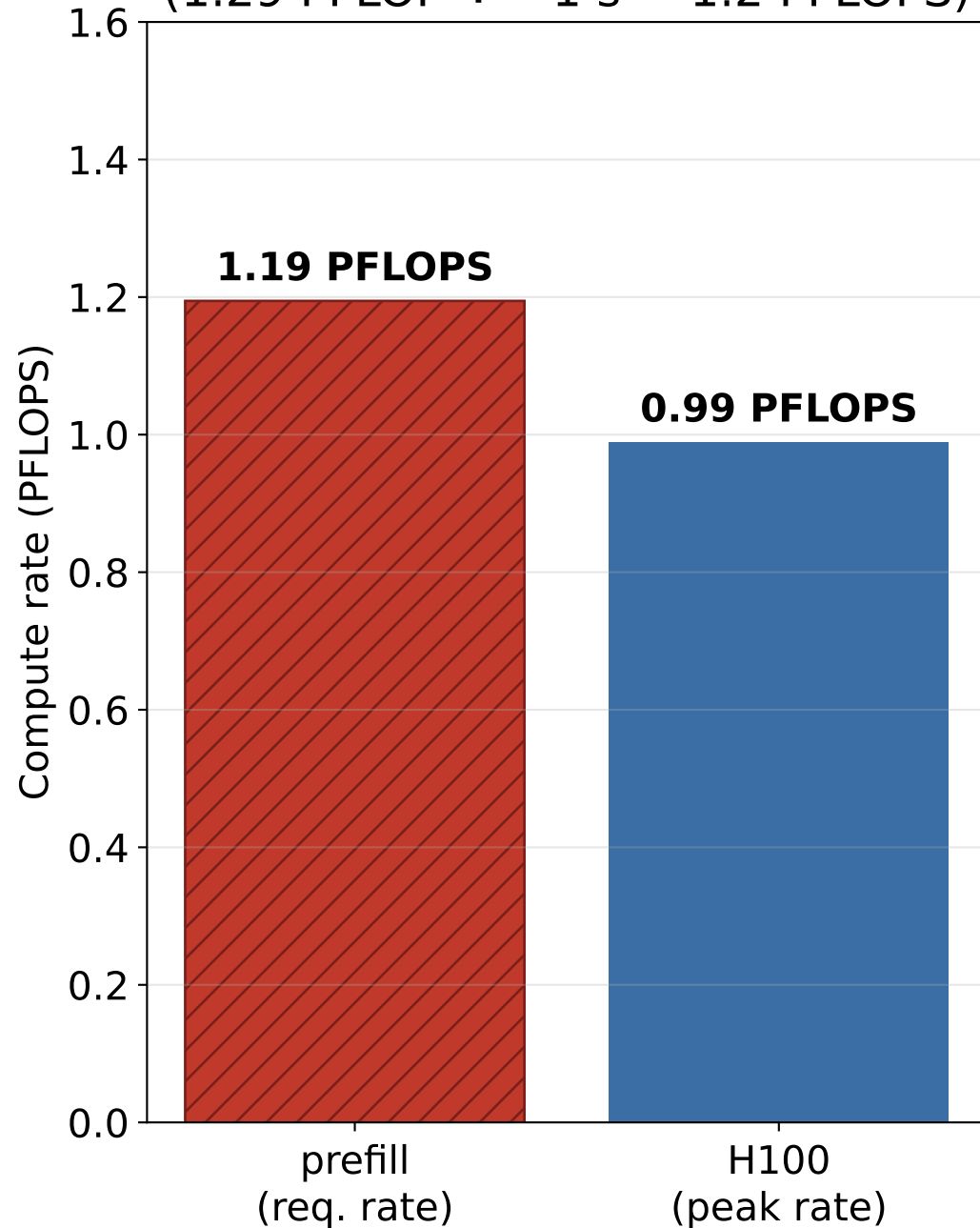
Prefill: compute-bound \rightarrow required rate (1.29 PFLOP \div \sim 1 s \approx 1.2 PFLOPS)
