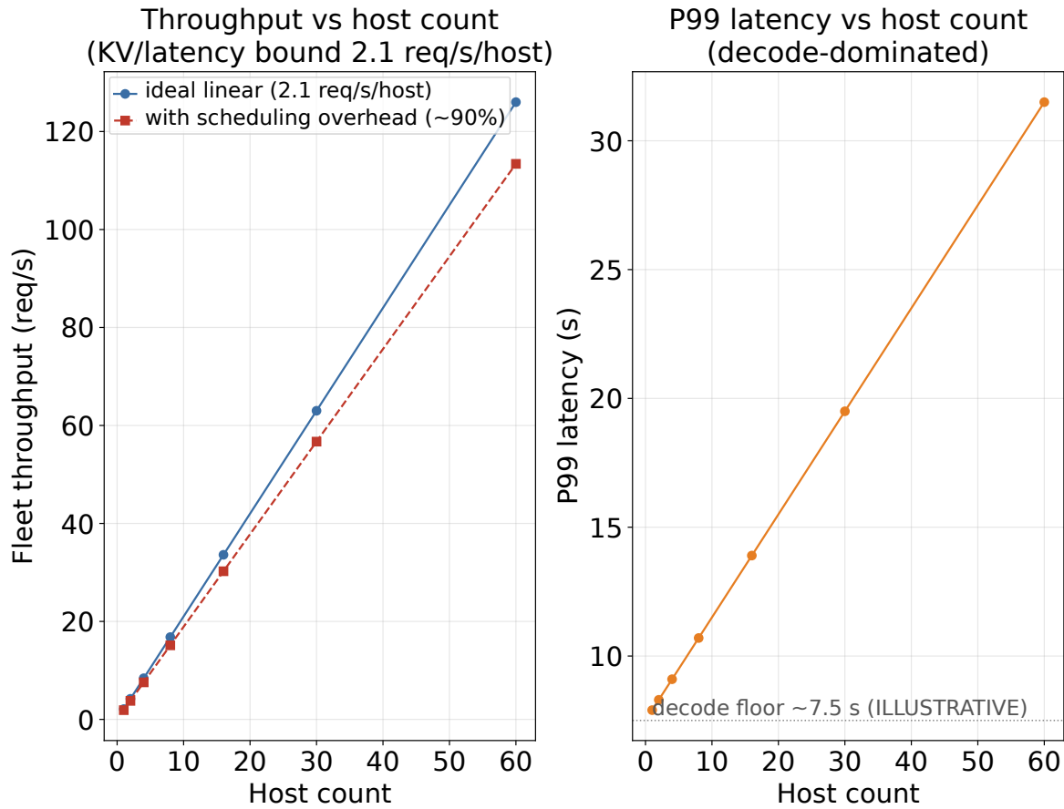
FIGURE 20.1: Fleet QPS and latency vs. host count, batch size, and scheduling overhead [ILLUSTRATIVE][DERIVED]
