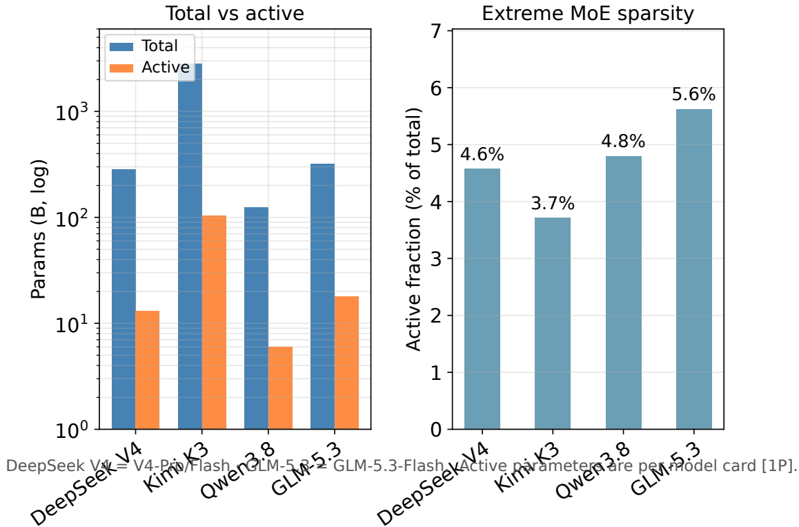
FIGURE A.1: 2026 frontier MoE extreme sparsity: four open models, total vs activated parameters, and active fraction in single digits [1P]
