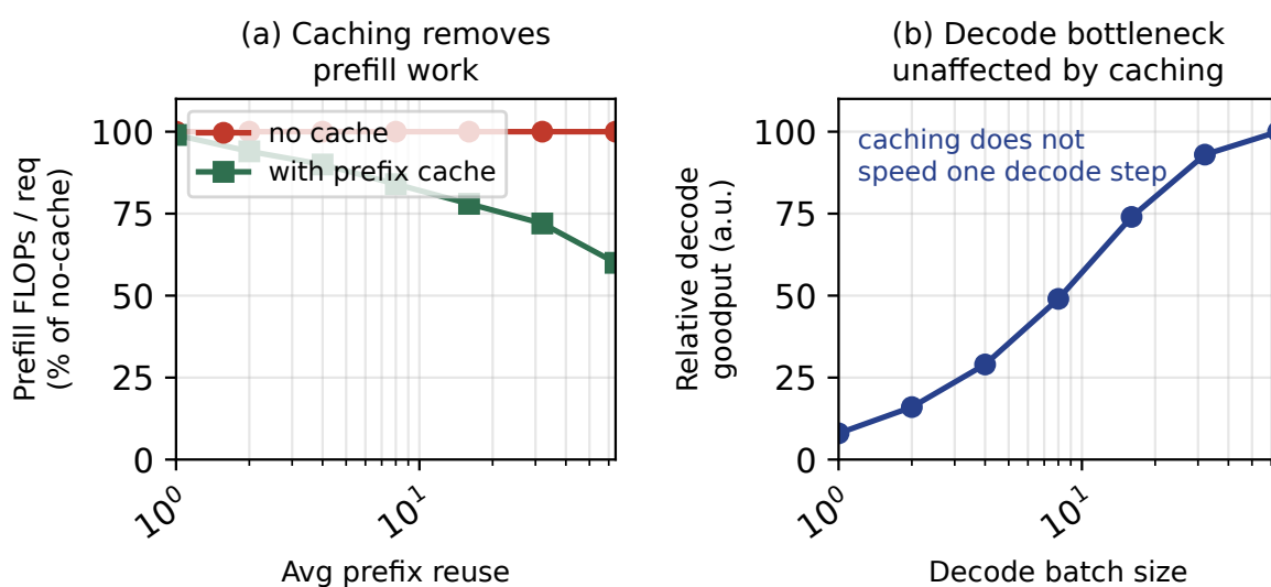
FIGURE 15.2: Prefix caching and batching affect different serving phases: caching reduces prefill work; batching raises decode goodput
