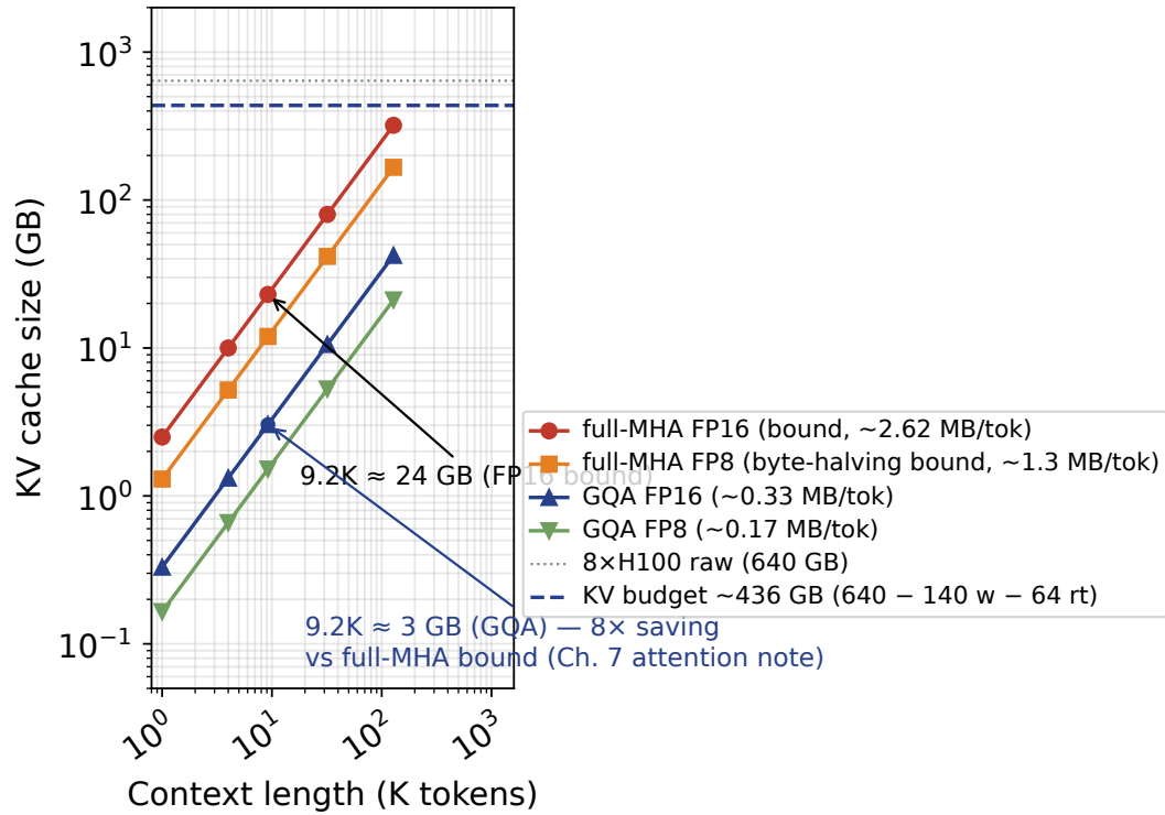
FIGURE 7.2: KV cache size vs context length for the canonical 80-layer reference geometry: full-MHA vs GQA (and FP8/8-bit). Note the broader lesson this title encodes: parameter count does not determine KV size . KV per token depends on layers \times KV-head count \times head dimension \times precision — i.e. on the attention shape , not on the number of parameters. A 70B full-MHA model and a 70B GQA model have very different KV footprints; the full-MHA curve is the conservative upper-bound teaching baseline, the GQA curve the \sim 8\times reduction. Parameter count is only a proxy for weight residency and rough dense FLOPs, never for KV footprint. [ILLUSTRATIVE][DERIVED]
