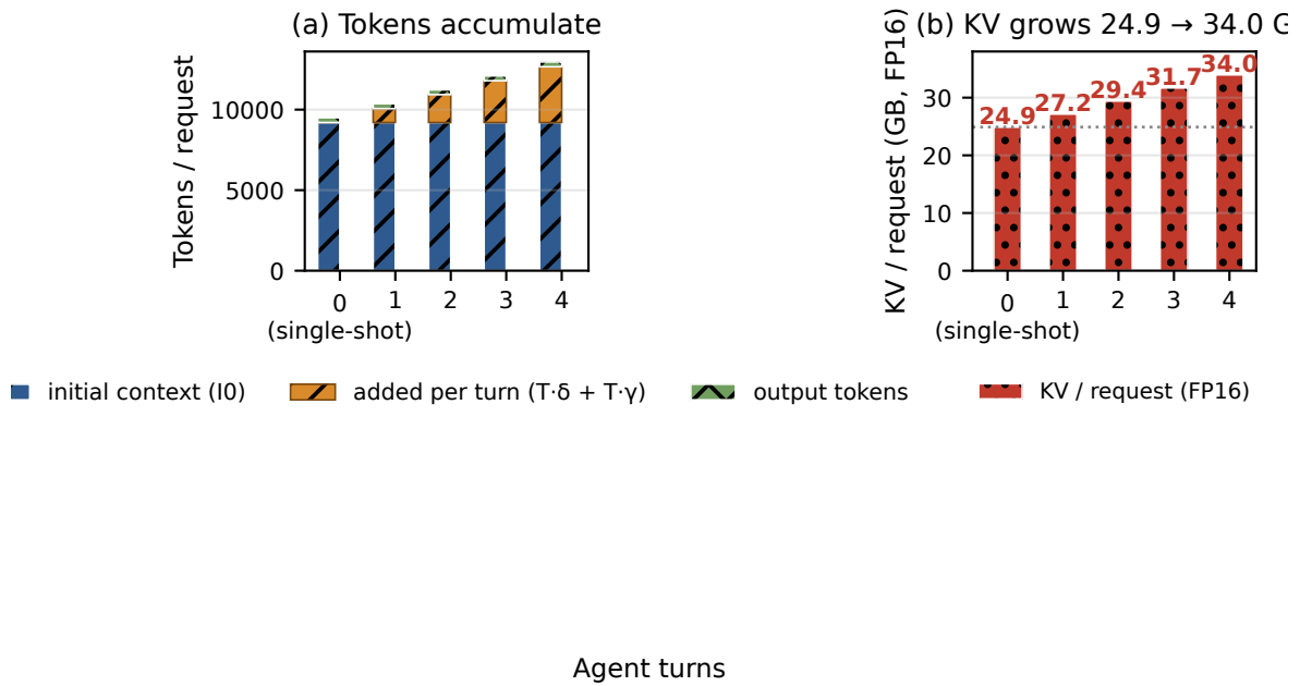
FIGURE 19.2: Input/output tokens and KV cache per request across agent turns ( I_0 + T \cdot \delta + T \cdot \gamma + O_{\text{final}} ; 9,200 input + 300 output + 800 + 65 per turn), FP16 KV rising from 24.9 GB single-shot to 34.0 GB at 4 turns. This chart quantifies the growth — the total token and KV numbers as turns accumulate. (Companion Fig 19.3 shows the mechanism of why it grows.) [DERIVED: Ch19 §3 arithmetic]
