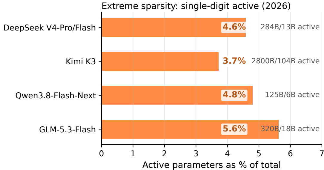
FIGURE A.1: 2026 frontier MoE extreme sparsity: four open models, total vs activated parameters, and active fraction in single digits [1P]
