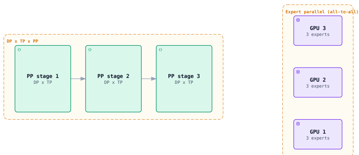
FIGURE 10.1. Fig 10.1 — Composing the dimensions: each PP stage holds a DP replica, TP-sharded across GPUs; and EP's per-token all-to-all routes each token to the GPU holding its experts (ILLUSTRATIVE)
