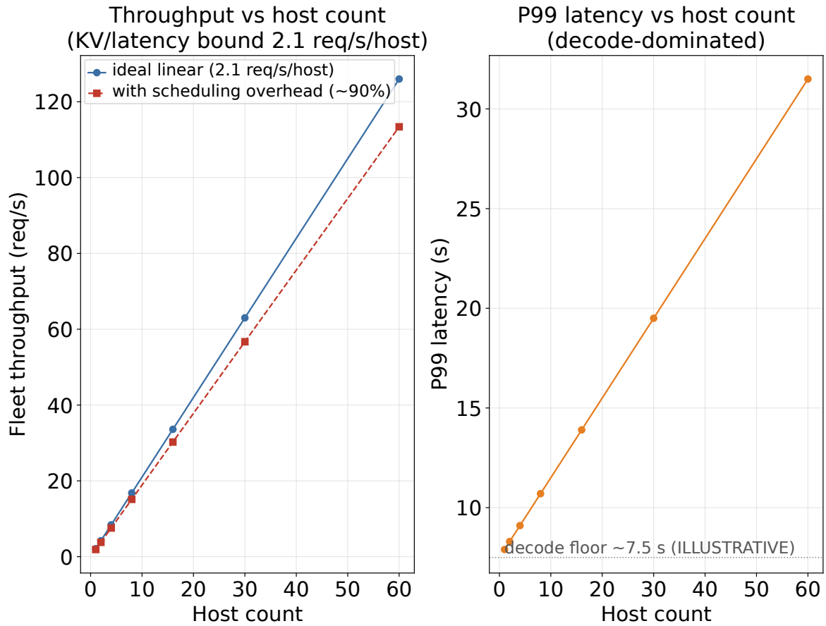
FIGURE 20.1: Fleet QPS and latency vs. host count, batch size, and scheduling overhead [ILLUSTRATIVE][DERIVED]
