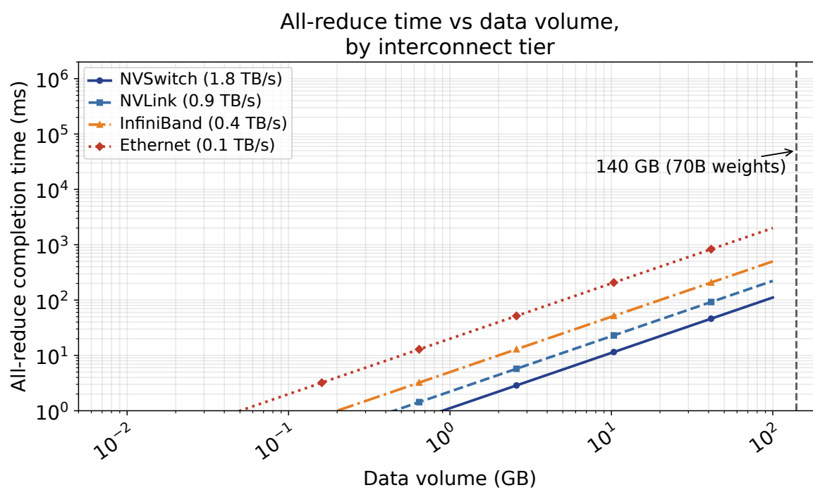
FIGURE 9.1: All-reduce time vs data volume, by interconnect tier [1P][DERIVED]
