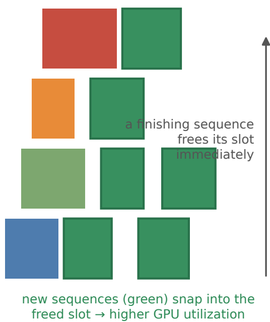
FIGURE 11.1: Discrete vs continuous batching (Orca-style slot diagram)
