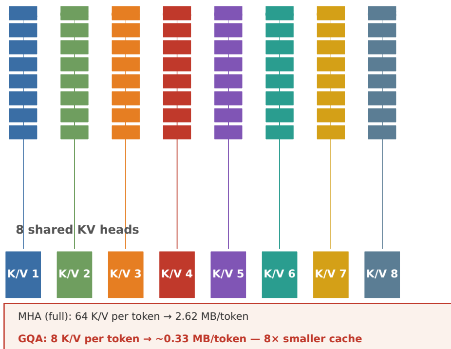
FIGURE 7.1: Grouped-Query Attention cuts per-token KV
