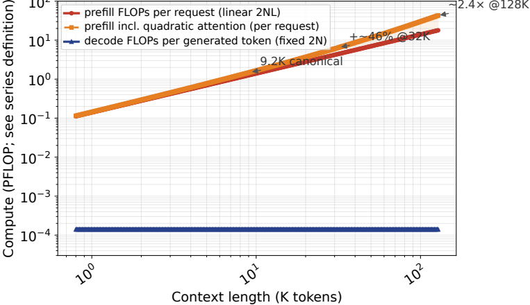
Full-attention prefill increasingly reflects quadratic attention cost; decode is incurred token-by-token
