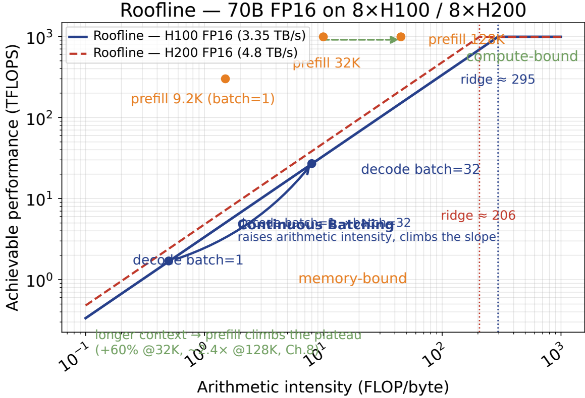
FIGURE 8.1: Prefill above the ridge (compute-bound), decode below it (memory-bound). H100 (solid) vs H200 (dashed) ridge points from vendor datasheets (989 TFLOPS dense, 3.35 / 4.8 TB/s); Continuous-Batching arrow shows decode climbing the slope as batch grows [DERIVED from 1P: vendor datasheet]
