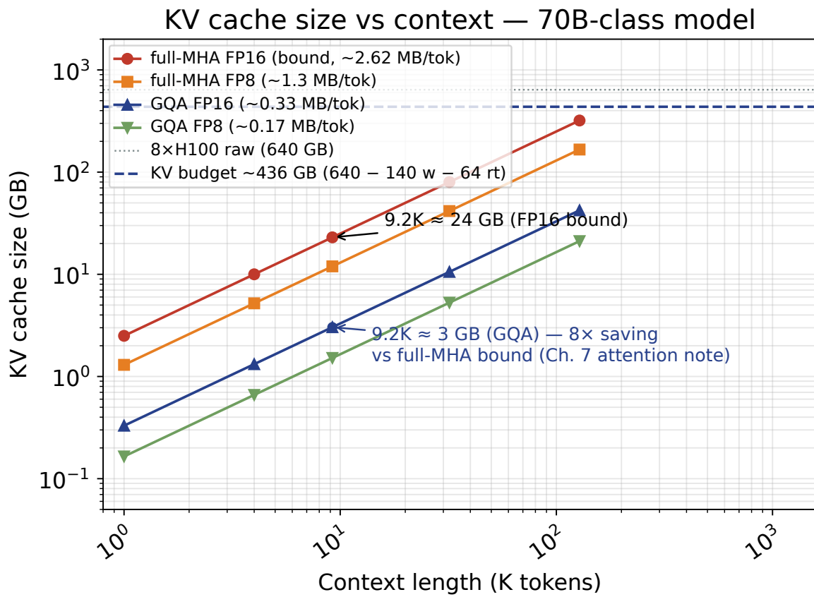
FIGURE 7.2: KV cache size vs context length for a 70B model [ILLUSTRATIVE][DERIVED]
