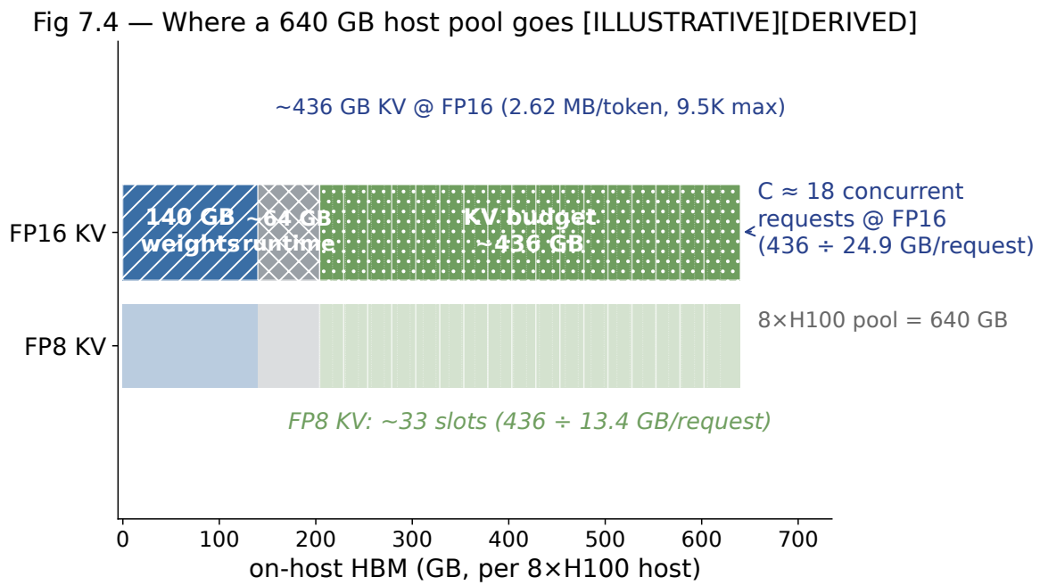
FIGURE 7.4: The concurrency budget: where a 70B host's 640 GB pool goes [ILLUSTRATIVE][DERIVED]
