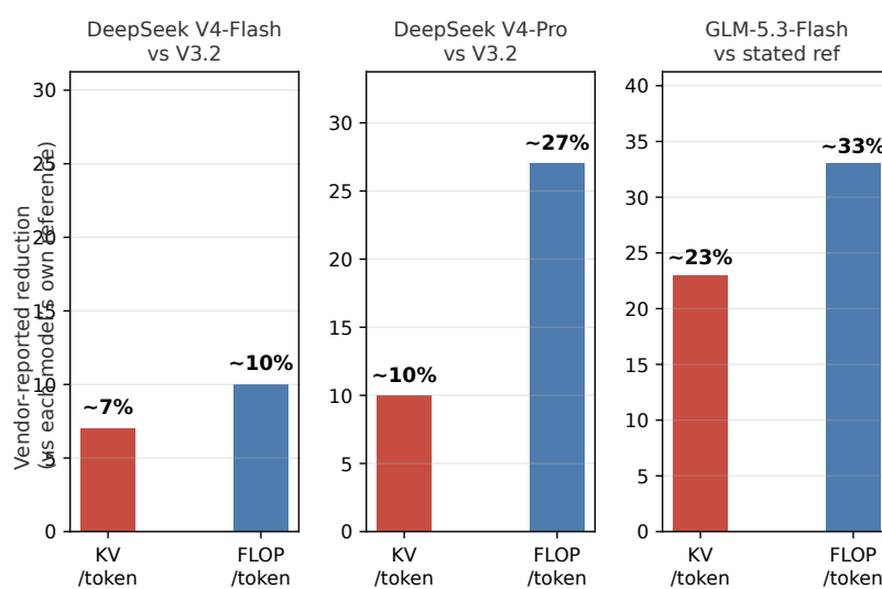
FIGURE A.2: Vendor-reported KV/FLOP reduction relative to each model's stated predecessor/reference, not a cross-model baseline [DERIVED from 1P claims: arXiv 2606.19348; HF zai-org]
