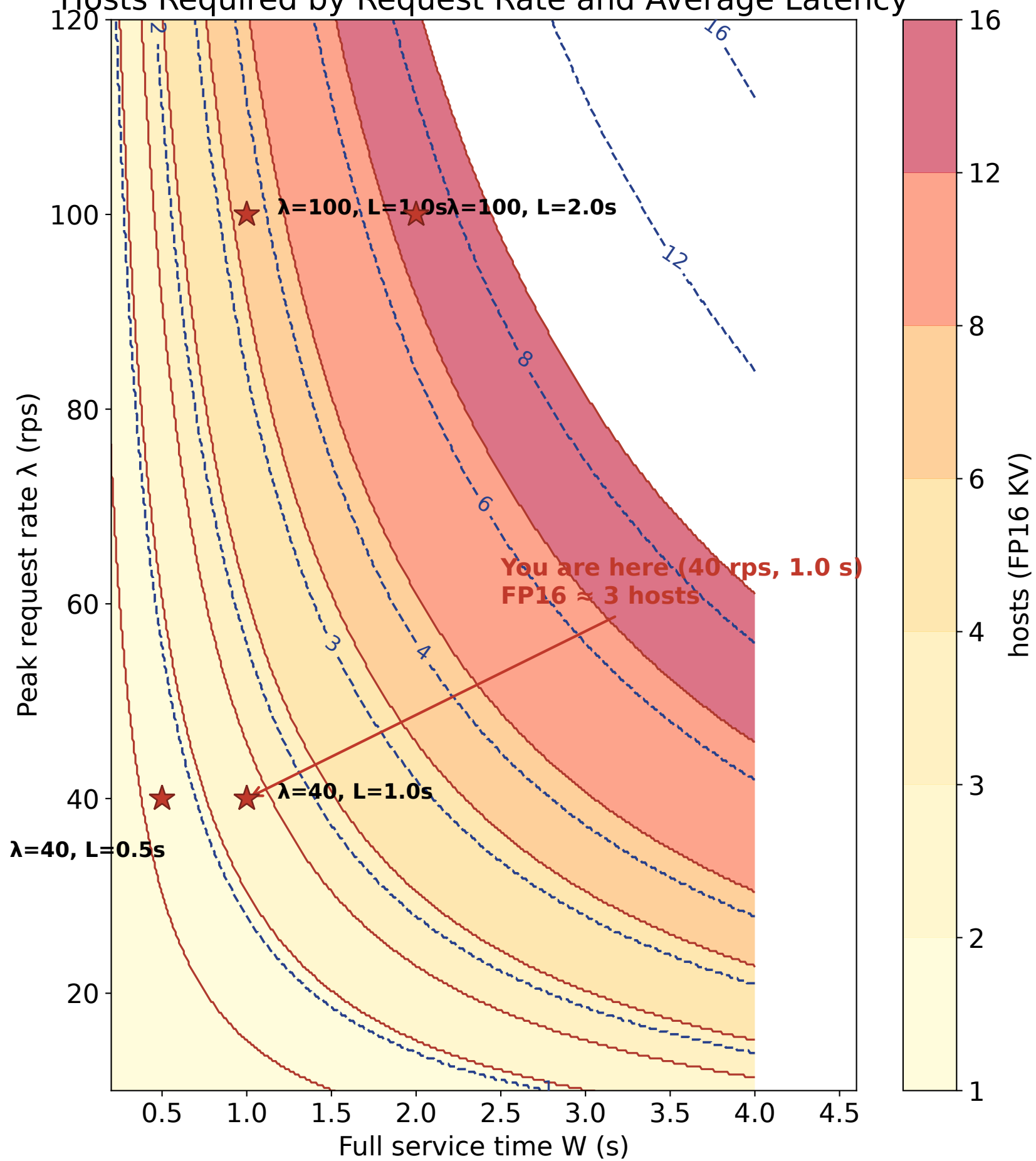
Hosts Required by Request Rate and Average Latency
