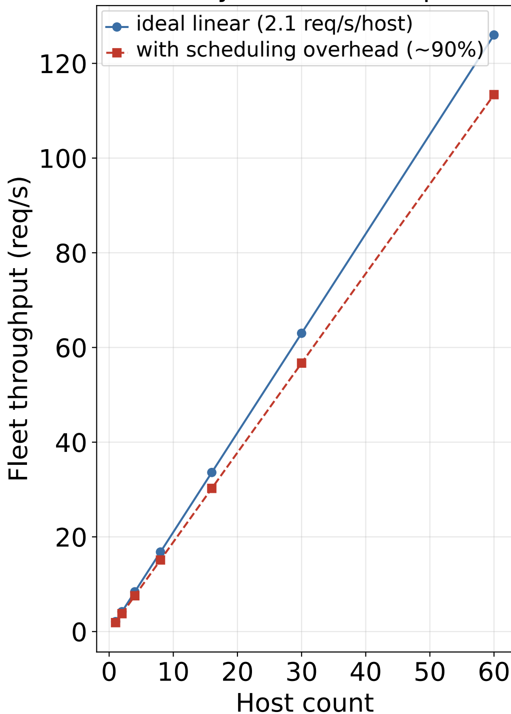
Throughput vs host count (KV/latency bound 2.1 req/s/host)
