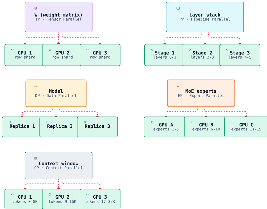
FIGURE 10.2. Fig 10.2 — The five parallelization strategies and what each splits [ILLUSTRATIVE conceptual]
