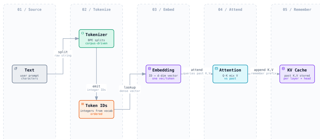
FIGURE 1.2. Fig 1.2 — How a token travels: text → tokenizer → IDs → embedding → attention → KV cache [ILLUSTRATIVE conceptual]
