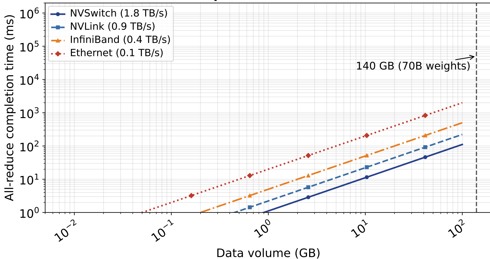
All-reduce time vs data volume, by interconnect tier
