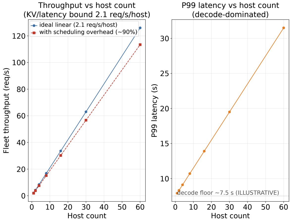
FIGURE 20.1: Fleet QPS and latency vs. host count, batch size, and scheduling overhead [2° DERIVED]
