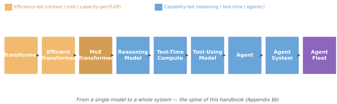
FIGURE A.3. Fig A.3 — The layered evolution of frontier systems, colour-coded by efficiency-led (amber) vs capability-led (blue) stages, from a single Transformer to the whole fleet (Appendix §6)
