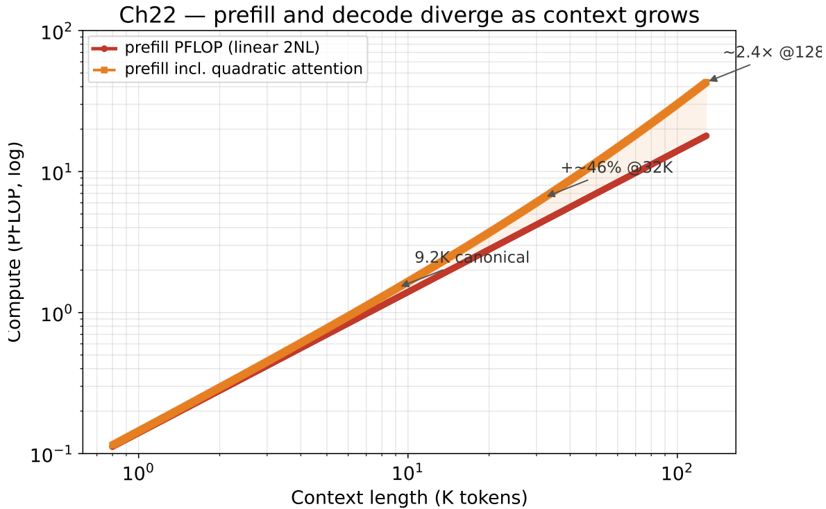
FIGURE 22.1. Fig 22.1 - Prefill vs decode bottleneck divergence [2° DERIVED]
