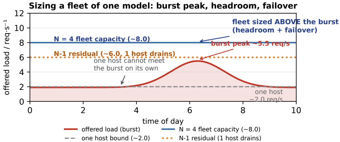
FIGURE 17.1: Sizing a fleet of one model by burst peak, headroom, and failover: offered load rises to a ~5.5 req/s burst that a single host (~2.0 req/s analytical planning bound) cannot meet; a 4-host fleet (~8.0 req/s at the analytical bound) is sized ABOVE the burst, and after one host drains the N-1 = 3 residual (~6.0 req/s) still clears it [ILLUSTRATIVE][DERIVED]
