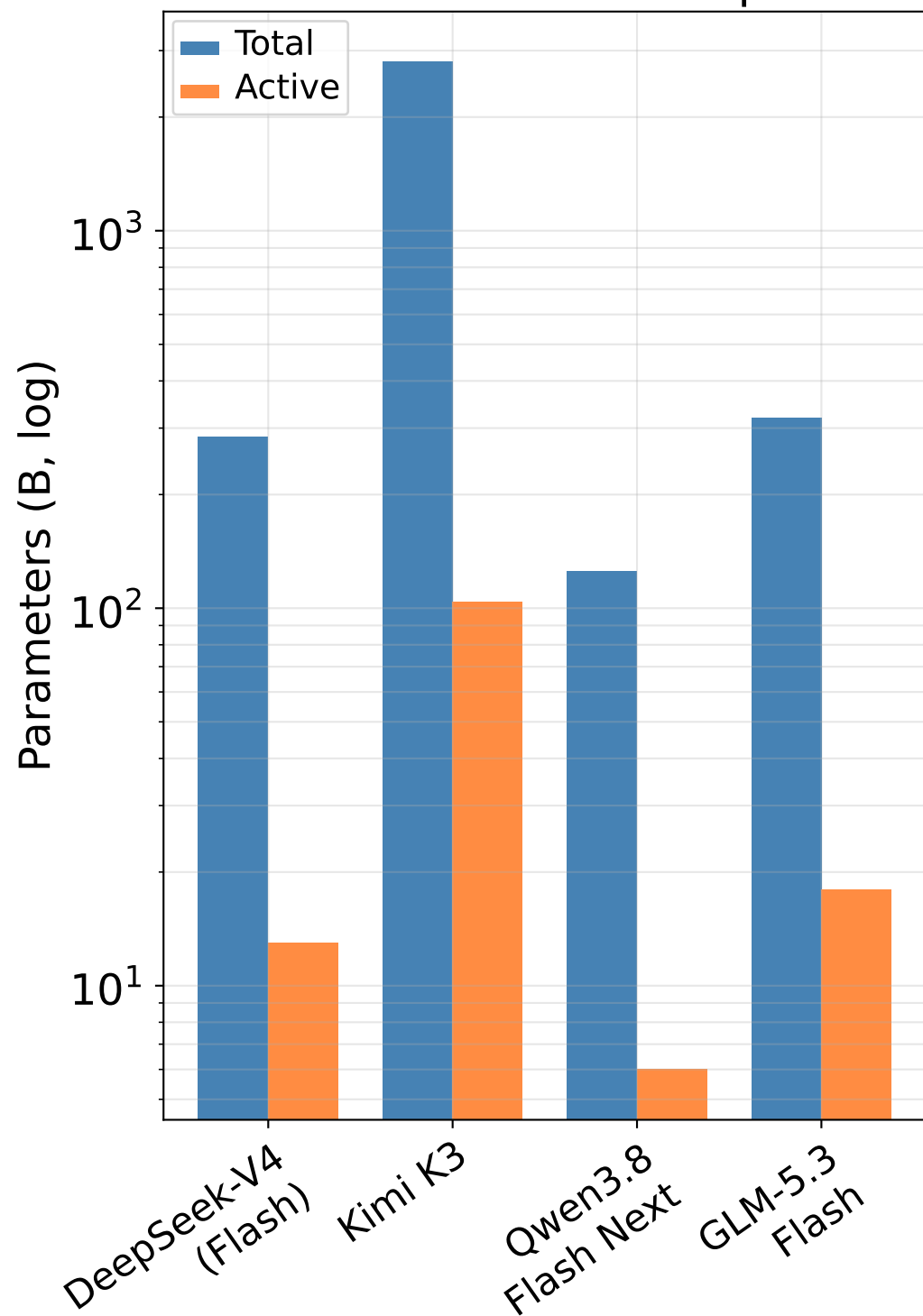
Frontier MoE: total vs active params [1P] Extreme MoE sparsity — single digits
