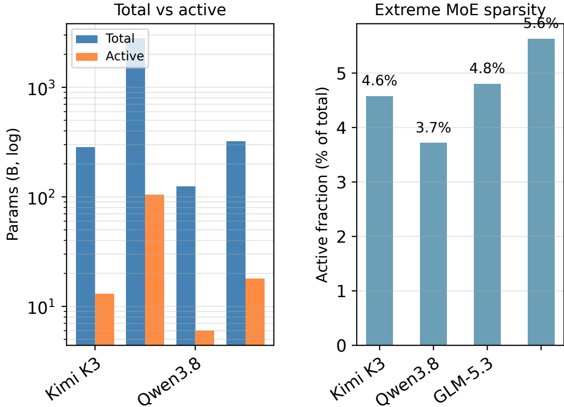
FIGURE A.1: 2026 frontier MoE extreme sparsity: four open models, total vs activated parameters, and active fraction in single digits [1P]
