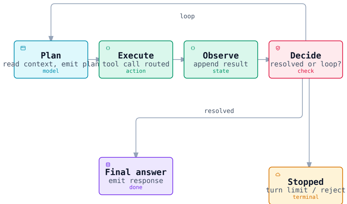
FIGURE 19.1. Fig 19.1 - The agent loop as a four-state state machine (Plan, Execute, Observe, Decide) with a loop-back to Plan and the terminal outcomes final answer and stopped [ILLUSTRATIVE conceptual]
