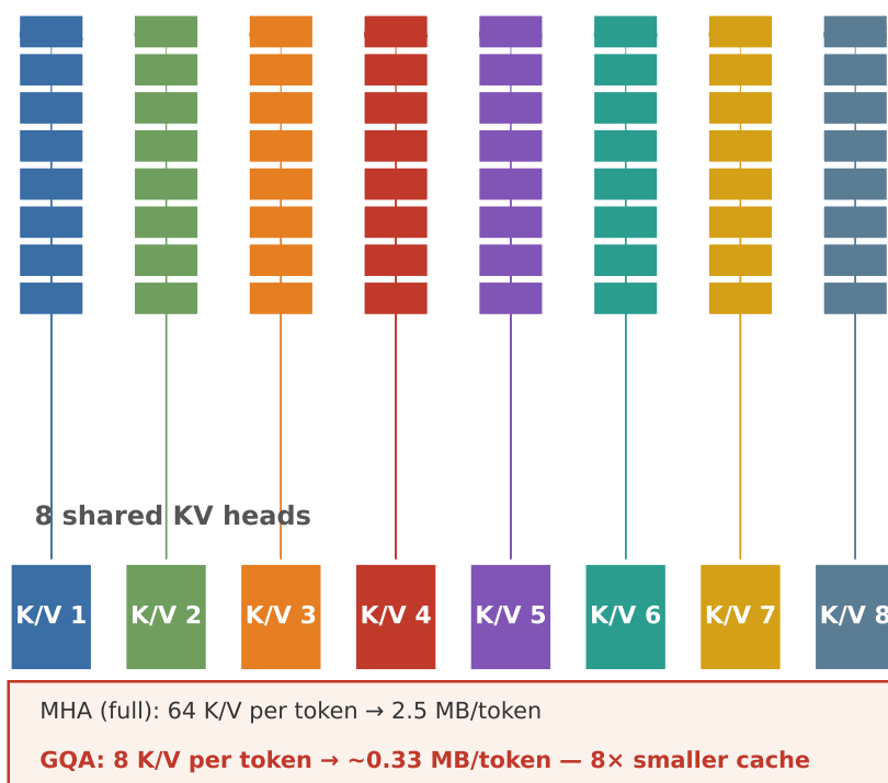
FIGURE 7.1. Fig 7.1 — Grouped-Query Attention: 64 query heads share 8 KV heads, cutting per-token KV 8× from 2.5 MB to ~0.33 MB (ILLUSTRATIVE, after LLaMA-2 70B head layout)
