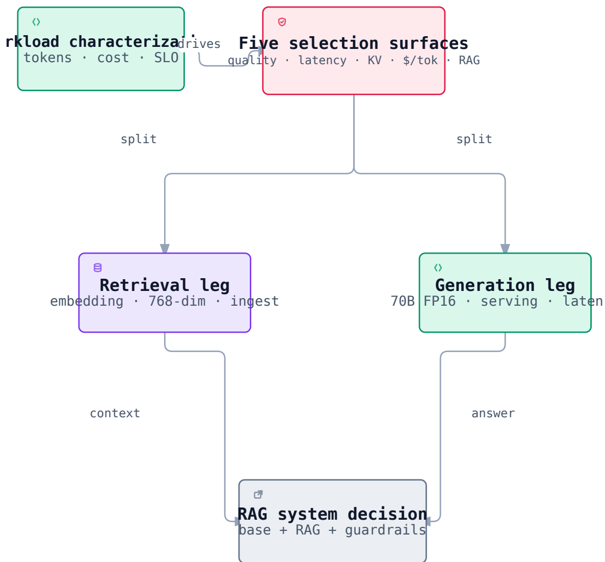
FIGURE 5.1. Fig 5.1 — Model selection for RAG: workload → five selection surfaces → two legs (retrieval/embedding, generation/70B) → the system decision [ILLUSTRATIVE conceptual]
