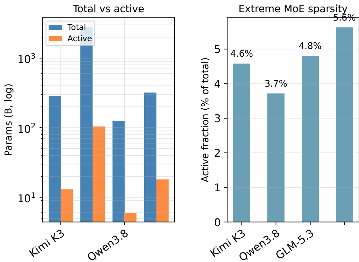
FIGURE A.1: 2026 frontier MoE extreme sparsity: four open models, total vs activated parameters, and active fraction in single digits [1P]
