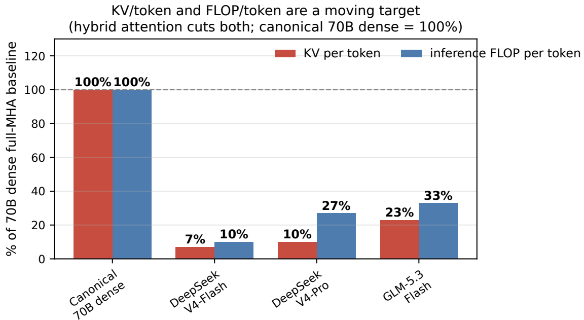
FIGURE A.2: The KV constant and FLOP/token are a moving target: hybrid attention cuts both at the mechanism. Canonical 70B dense full-MHA = 100%; DeepSeek-V4-Flash \approx 7% KV / 10% FLOP, V4-Pro \approx 10% / 27%, GLM-5.3-Flash \approx 23% KV / \sim 33% attention-compute
