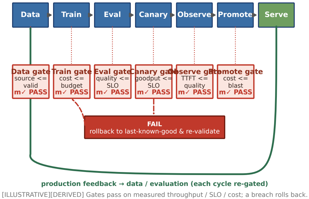
FIGURE 21.1: The AI Factory promotion pipeline [ILLUSTRATIVE conceptual]
