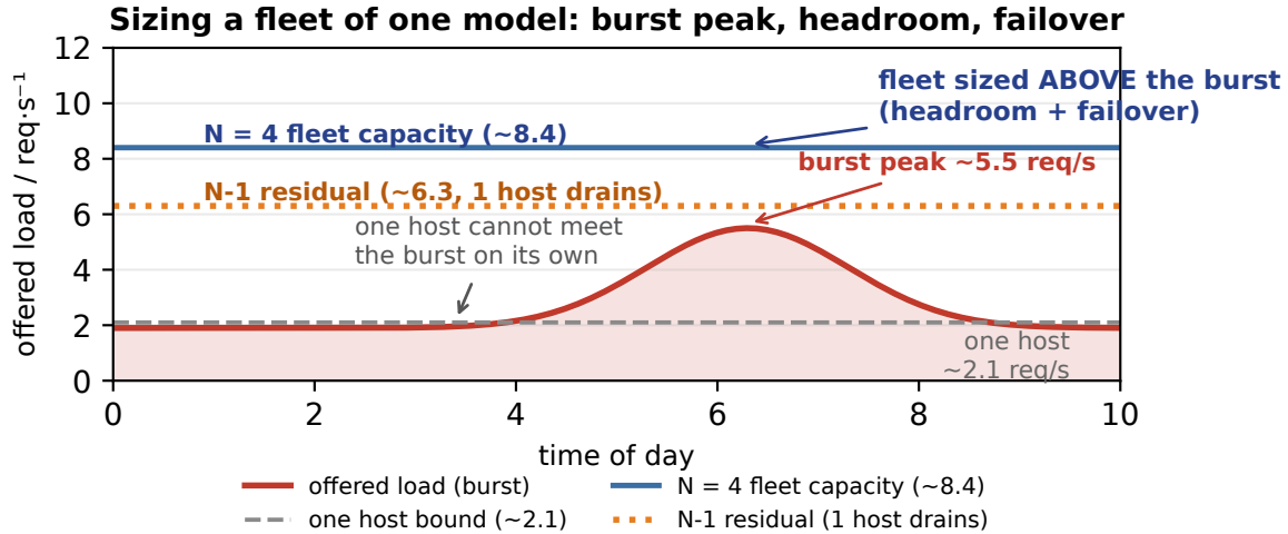
FIGURE 17.1: Sizing a fleet of one model by burst peak, headroom, and failover: offered load rises to a ~5.5 req/s burst that a single host (~2.1 req/s analytical service bound) cannot meet; a 4-host fleet (~8.4 req/s at the analytical bound) is sized ABOVE the burst, and after one host drains the N-1 = 3 residual (~6.3 req/s) still clears it [ILLUSTRATIVE][DERIVED]
