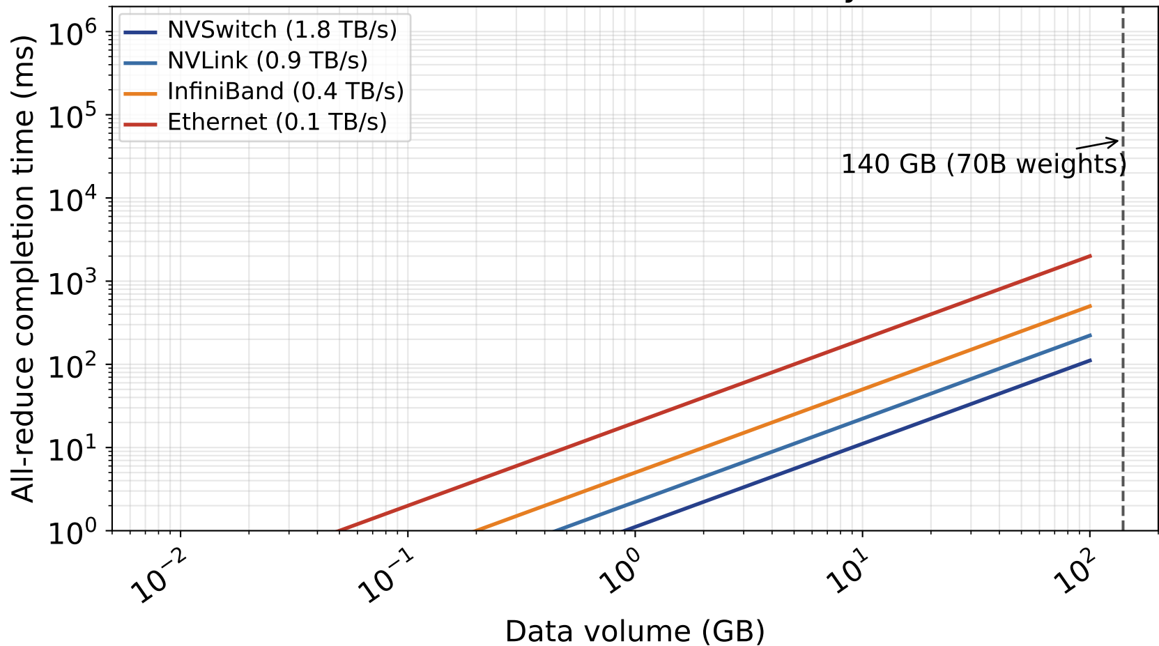
Ch09 — all-reduce time vs data volume, by interconnect tier
