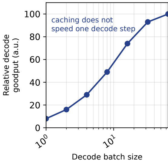
(b) Decode bottleneck unaffected by caching
