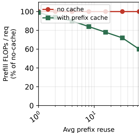
(a) Caching removes prefill work
