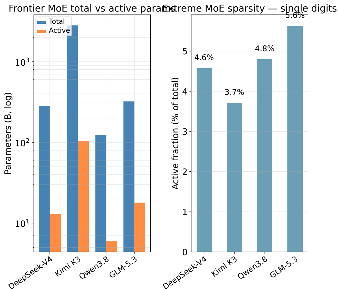
FIGURE A.1: 2026 frontier MoE extreme sparsity: four open models, total vs activated parameters, and active fraction in single digits [1P]
