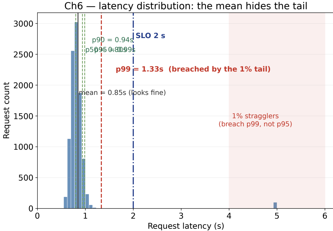
FIGURE 6.2: Request-latency distribution: p50/p90/p95/p99 and the mean. The mean (~0.84 s) hides the 1% stragglers at ~5 s; it is the p99 budget (not p95) they breach (illustrative)
