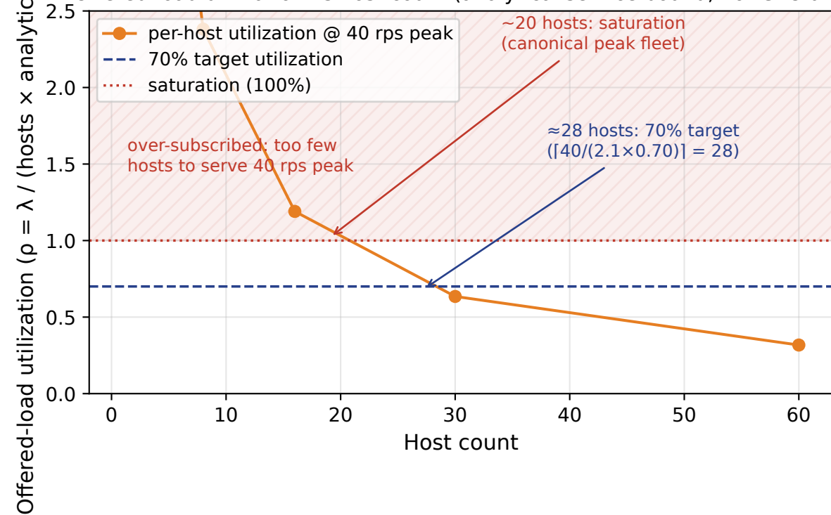
Offered-load utilization vs host count (analytical service bound, not GPU util)
