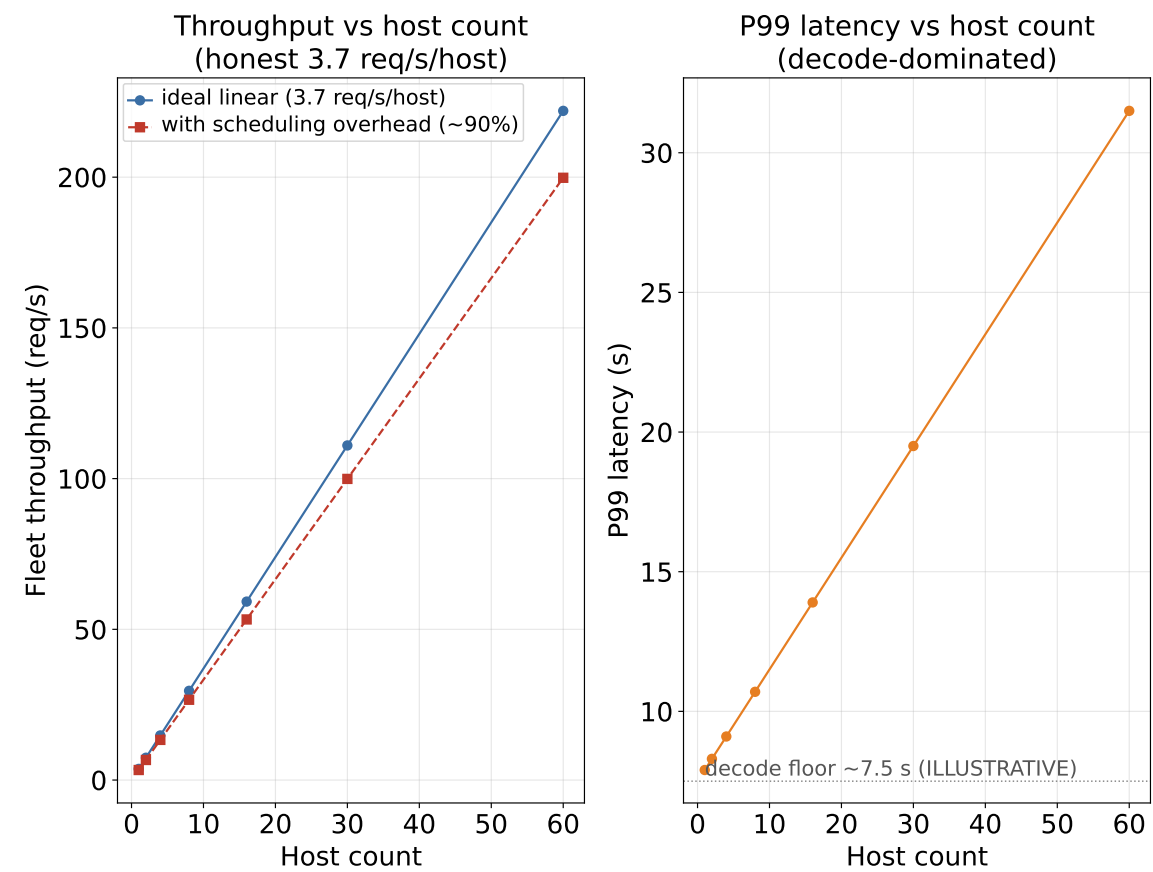
FIGURE 20.1. Fig 20.1 - Fleet QPS and latency vs. host count, batch size, and scheduling overhead [2° DERIVED]
