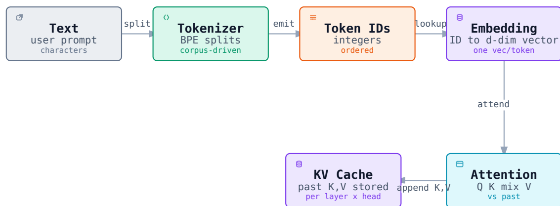
FIGURE 1.2. Fig 1.2 — How a token travels: text → tokenizer → IDs → embedding → attention → KV cache [ILLUSTRATIVE conceptual]
