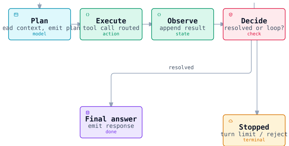
FIGURE 19.1. Fig 19.1 - The agent loop as a four-state state machine (Plan, Execute, Observe, Decide) with a loop-back to Plan and the terminal outcomes final answer and stopped [ILLUSTRATIVE conceptual]
